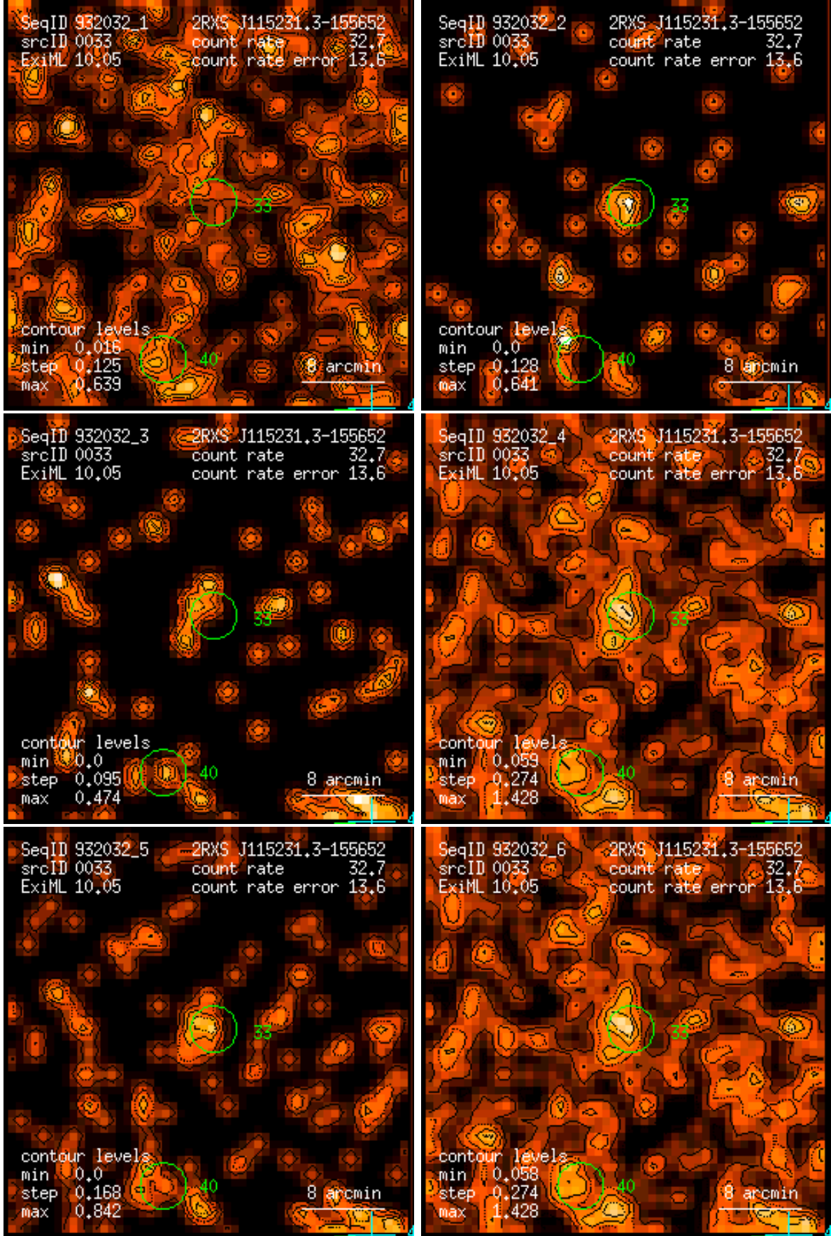
Figure 33: RASS 932032: detection 0033: band rate images, Gaussian filter: (1) PSPC channels 11 – 41, (2) 52 – 90, (3) 91 – 201, (4) 11 – 235, (5) 52 – 201, (6) 11 – 201. Broad band rates in counts/ks. Band rate contour levels in counts/ks/arcmin 2 .
