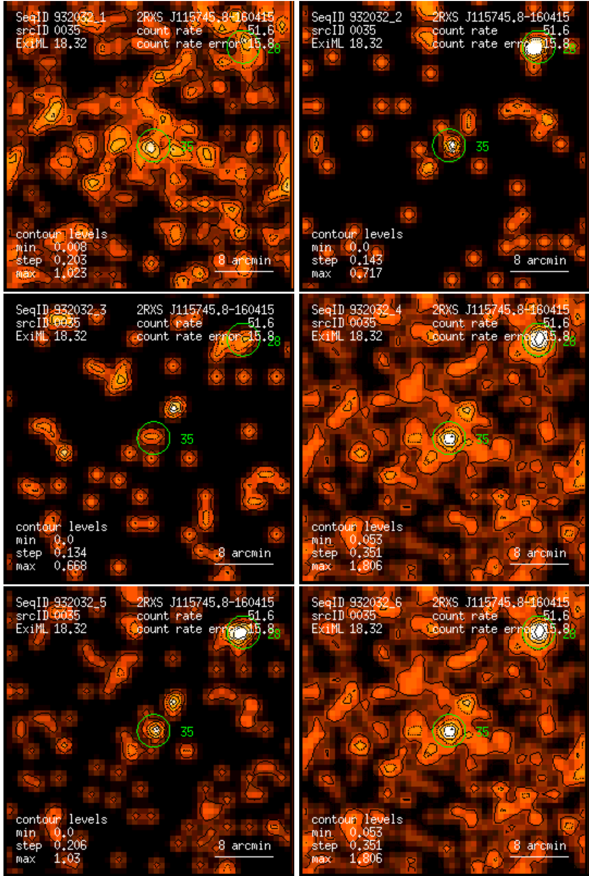
Figure 35: RASS 932032: detection 0035: band rate images, Gaussian filter: (1) PSPC channels 11 – 41, (2) 52 – 90, (3) 91 – 201, (4) 11 – 235, (5) 52 – 201, (6) 11 – 201. Broad band rates in counts/ks. Band rate contour levels in counts/ks/arcmin 2 .
