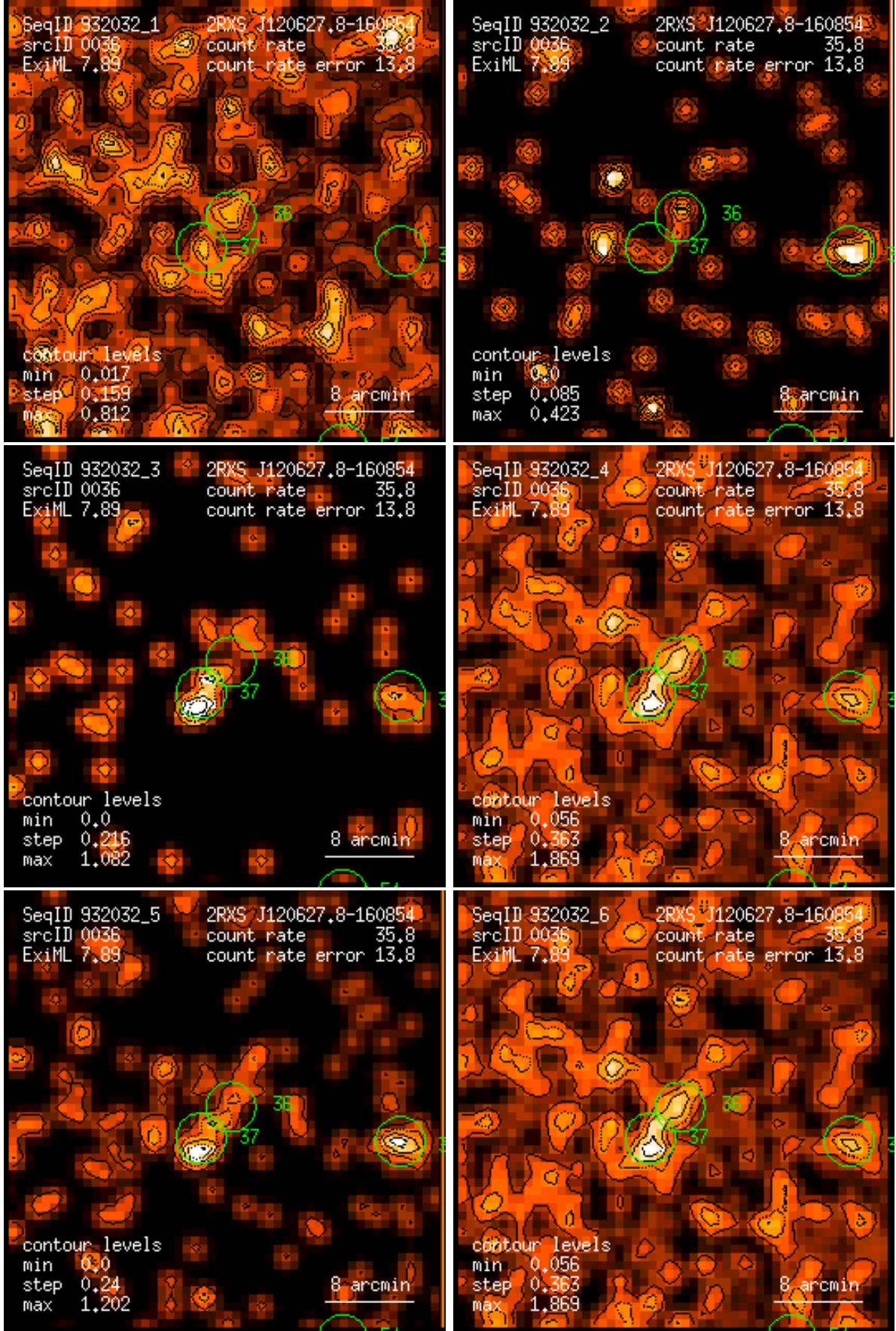
Figure 36: RASS 932032: detection 0036: band rate images, Gaussian filter: (1) PSPC channels 11 – 41, (2) 52 – 90, (3) 91 – 201, (4) 11 – 235, (5) 52 – 201, (6) 11 – 201. Broad band rates in counts/ks. Band rate contour levels in counts/ks/arcmin 2 .
