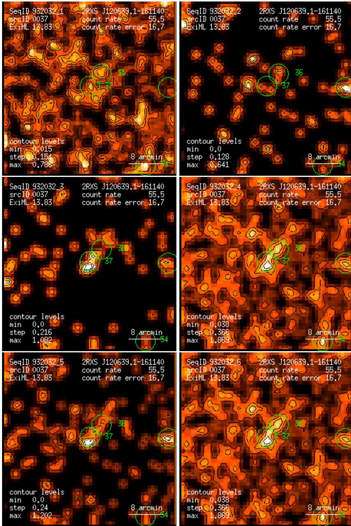
Figure 37: RASS 932032: detection 0037: band rate images, Gaussian filter: (1) PSPC channels 11 – 41, (2) 52 – 90, (3) 91 – 201, (4) 11 – 235, (5) 52 – 201, (6) 11 – 201. Broad band rates in counts/ks. Band rate contour levels in counts/ks/arcmin 2 .
