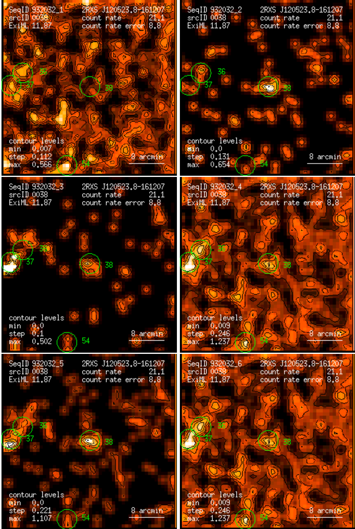
Figure 38: RASS 932032: detection 0038: band rate images, Gaussian filter: (1) PSPC channels 11 – 41, (2) 52 – 90, (3) 91 – 201, (4) 11 – 235, (5) 52 – 201, (6) 11 – 201. Broad band rates in counts/ks. Band rate contour levels in counts/ks/arcmin 2 .
