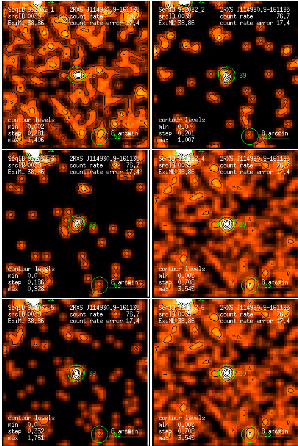
Figure 39: RASS 932032: detection 0039: band rate images, Gaussian filter: (1) PSPC channels 11 – 41, (2) 52 – 90, (3) 91 – 201, (4) 11 – 235, (5) 52 – 201, (6) 11 – 201. Broad band rates in counts/ks. Band rate contour levels in counts/ks/arcmin 2 .
