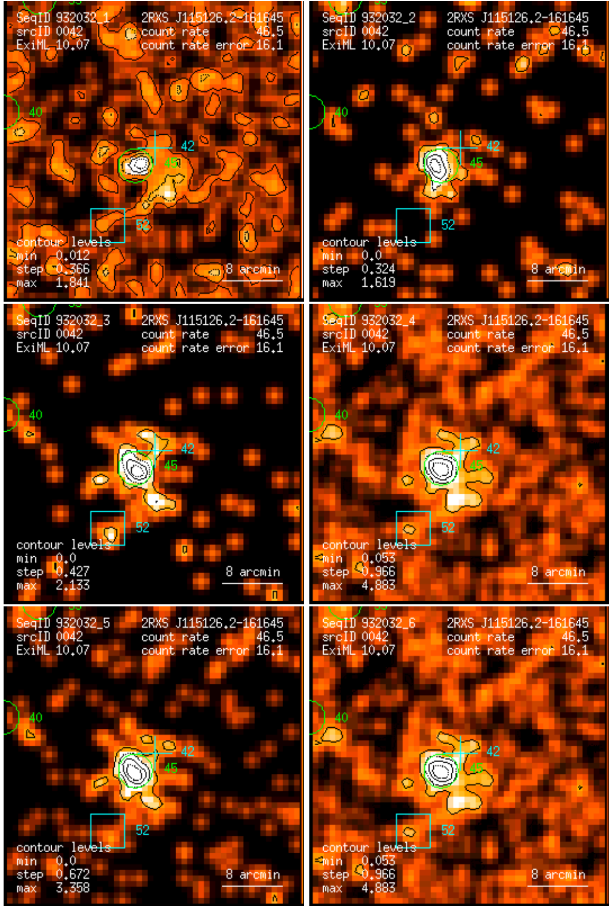
Figure 42: RASS 932032: detection 0042: band rate images, Gaussian filter: (1) PSPC channels 11 – 41, (2) 52 – 90, (3) 91 – 201, (4) 11 – 235, (5) 52 – 201, (6) 11 – 201. Broad band rates in counts/ks. Band rate contour levels in counts/ks/arcmin 2 .
