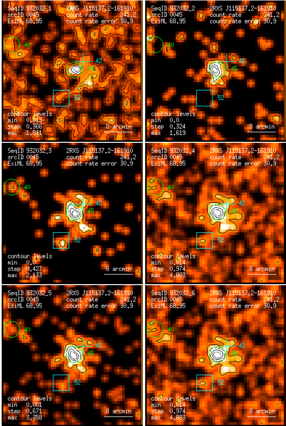
Figure 45: RASS 932032: detection 0045: band rate images, Gaussian filter: (1) PSPC channels 11 – 41, (2) 52 – 90, (3) 91 – 201, (4) 11 – 235, (5) 52 – 201, (6) 11 – 201. Broad band rates in counts/ks. Band rate contour levels in counts/ks/arcmin 2 .
