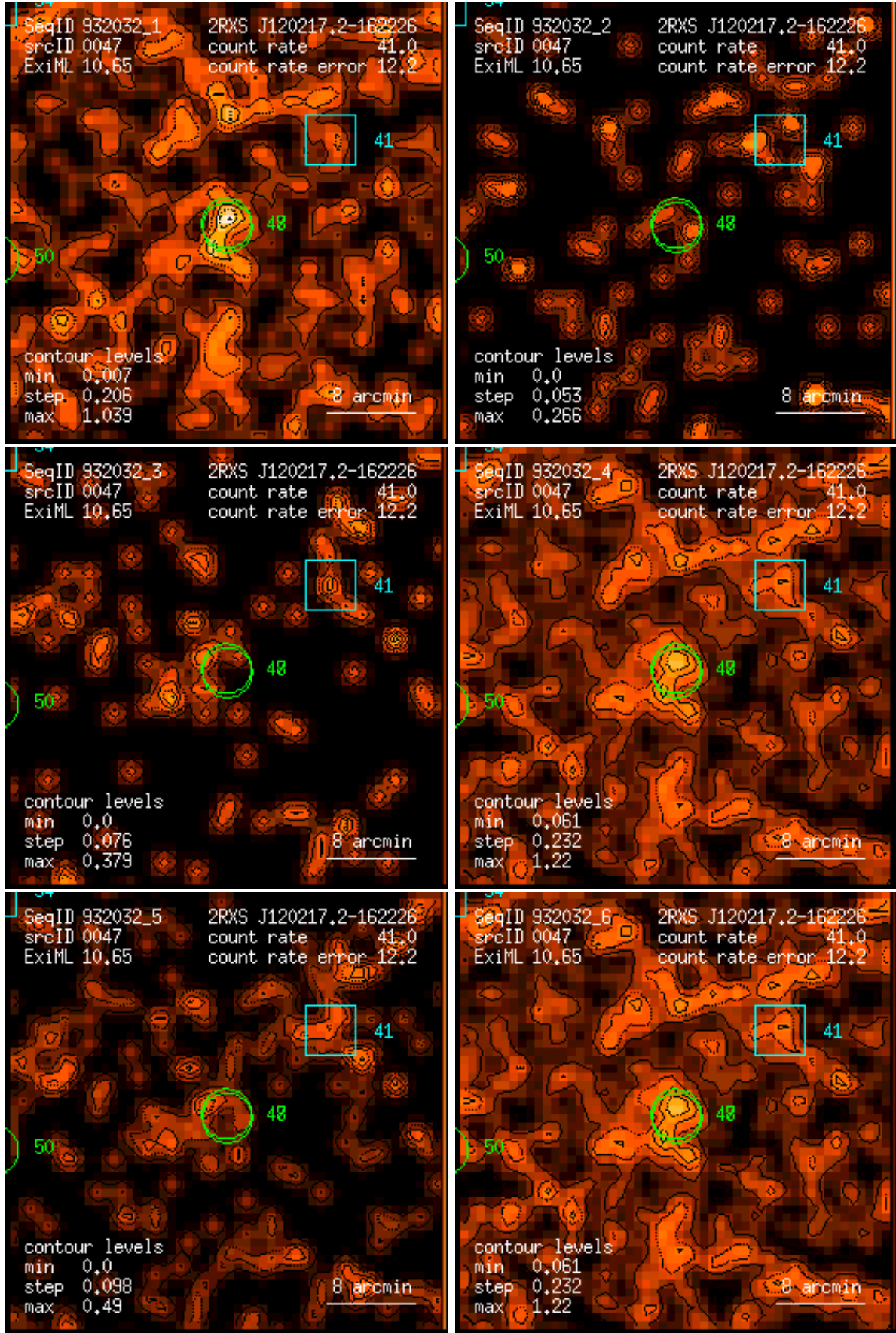
Figure 47: RASS 932032: detection 0047: band rate images, Gaussian filter: (1) PSPC channels 11 – 41, (2) 52 – 90, (3) 91 – 201, (4) 11 – 235, (5) 52 – 201, (6) 11 – 201. Broad band rates in counts/ks. Band rate contour levels in counts/ks/arcmin 2 .
