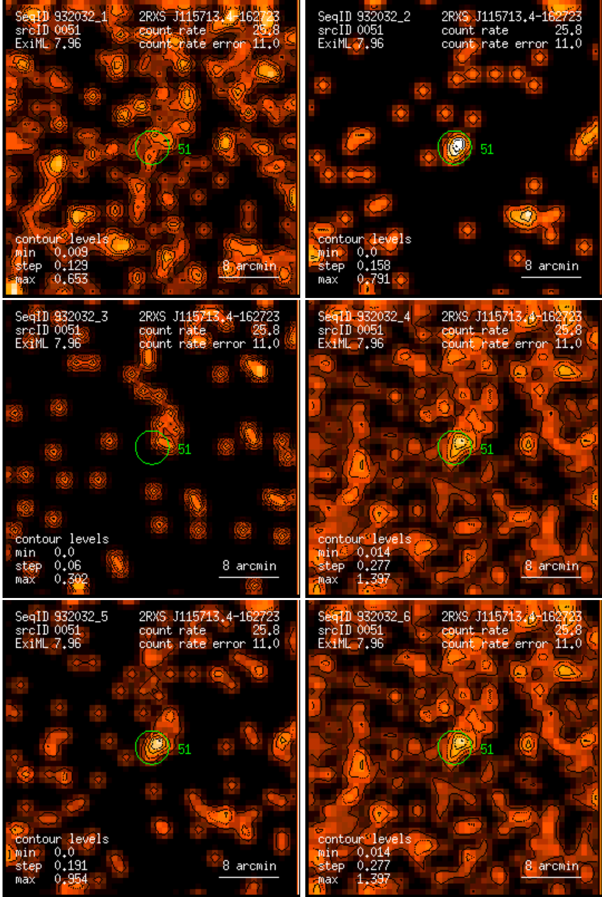
Figure 51: RASS 932032: detection 0051: band rate images, Gaussian filter: (1) PSPC channels 11 – 41, (2) 52 – 90, (3) 91 – 201, (4) 11 – 235, (5) 52 – 201, (6) 11 – 201. Broad band rates in counts/ks. Band rate contour levels in counts/ks/arcmin 2 .
