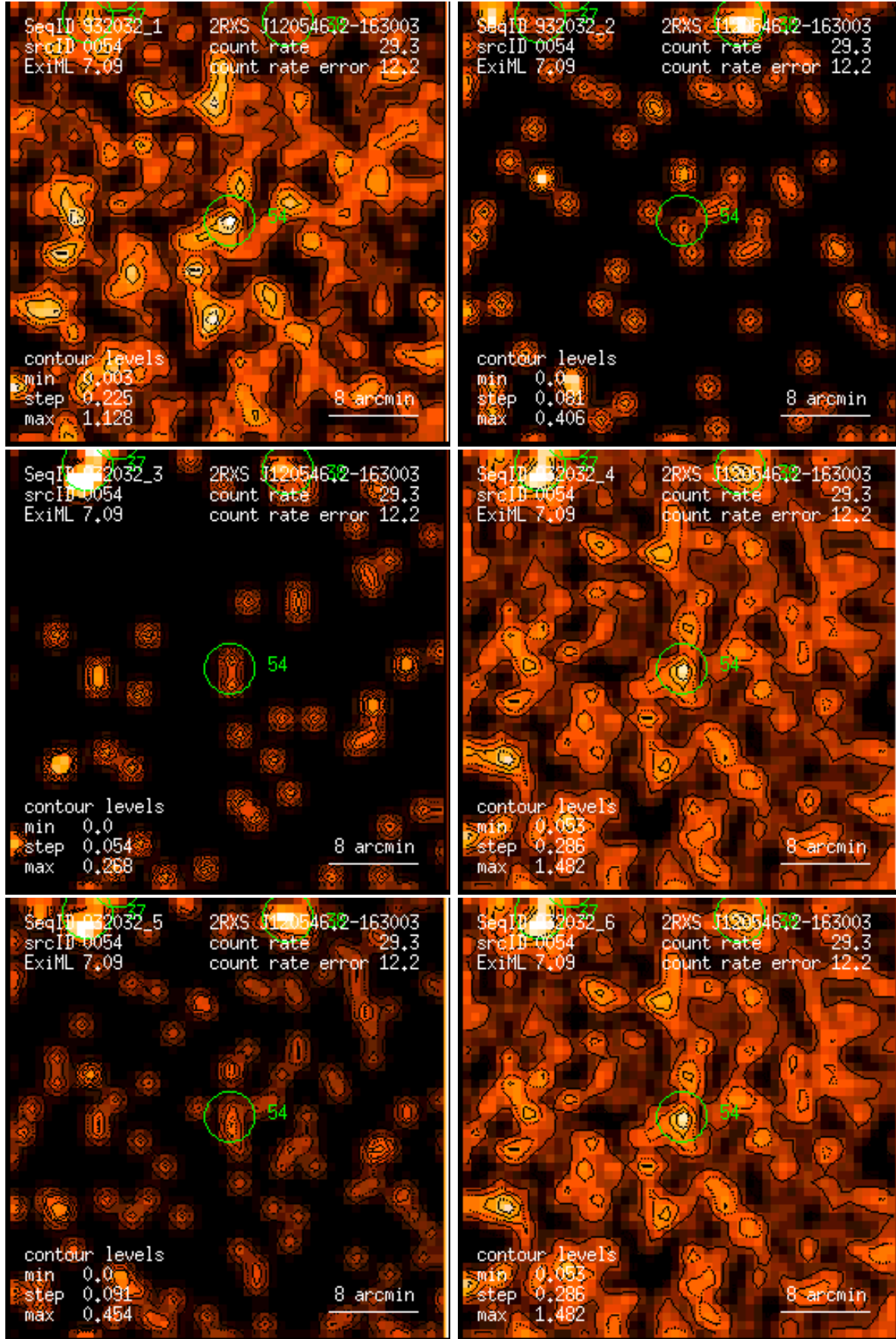
Figure 54: RASS 932032: detection 0054: band rate images, Gaussian filter: (1) PSPC channels 11 – 41, (2) 52 – 90, (3) 91 – 201, (4) 11 – 235, (5) 52 – 201, (6) 11 – 201. Broad band rates in counts/ks. Band rate contour levels in counts/ks/arcmin 2 .
