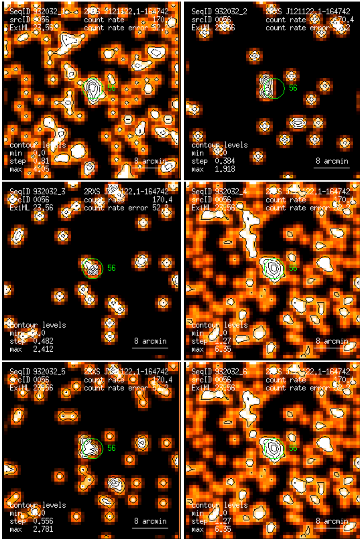
Figure 56: RASS 932032: detection 0056: band rate images, Gaussian filter: (1) PSPC channels 11 – 41, (2) 52 – 90, (3) 91 – 201, (4) 11 – 235, (5) 52 – 201, (6) 11 – 201. Broad band rates in counts/ks. Band rate contour levels in counts/ks/arcmin 2 .
