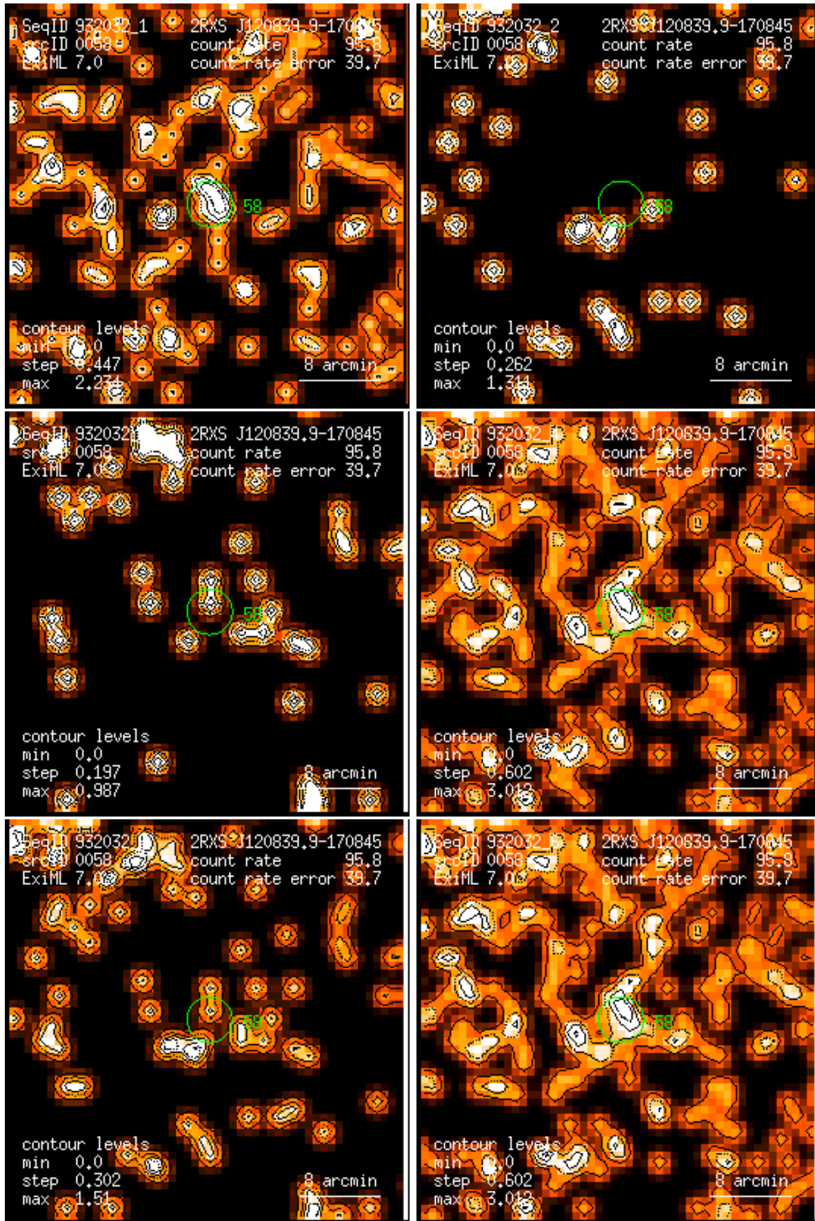
Figure 58: RASS 932032: detection 0058: band rate images, Gaussian filter: (1) PSPC channels 11 – 41, (2) 52 – 90, (3) 91 – 201, (4) 11 – 235, (5) 52 – 201, (6) 11 – 201. Broad band rates in counts/ks. Band rate contour levels in counts/ks/arcmin 2 .
