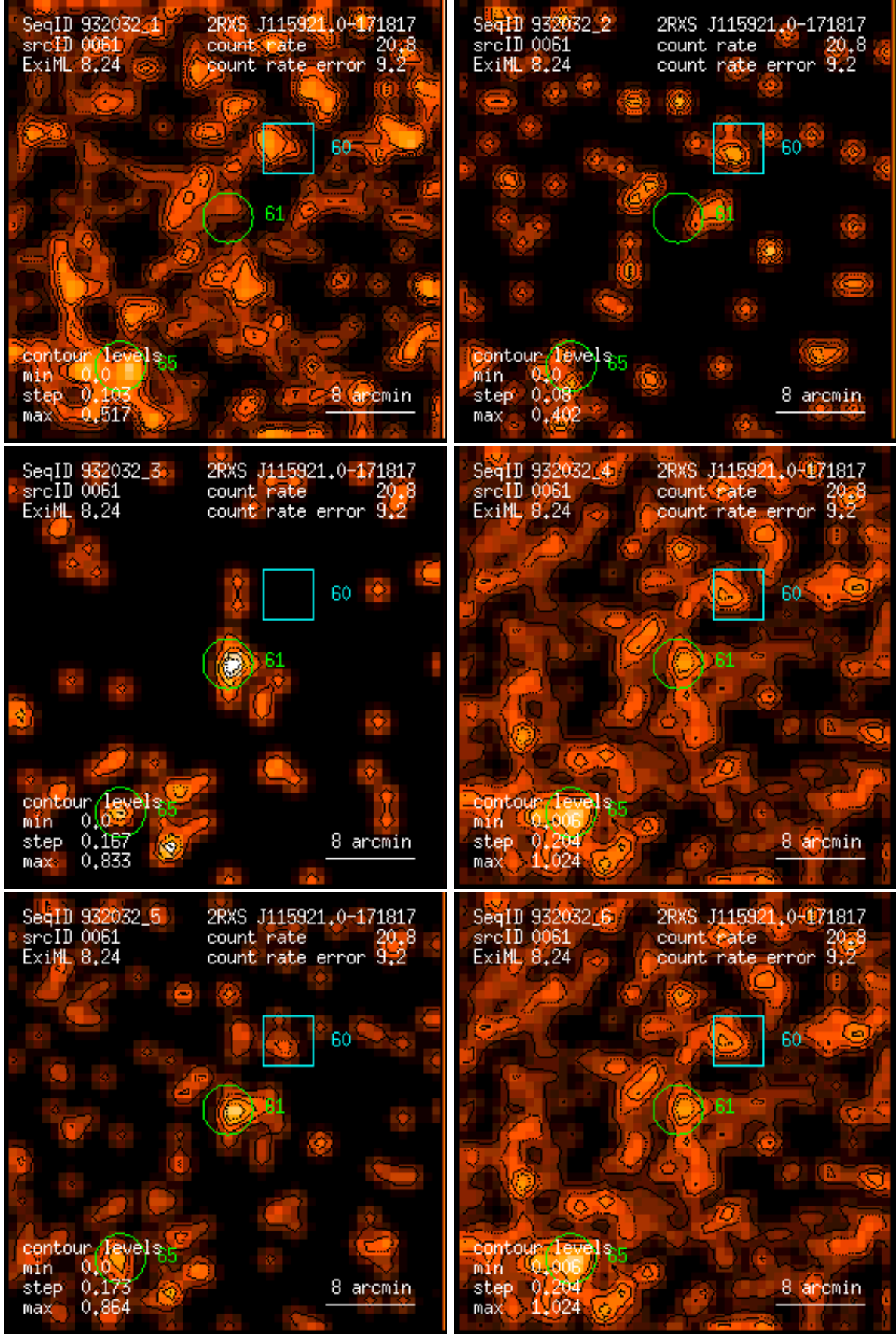
Figure 61: RASS 932032: detection 0061: band rate images, Gaussian filter: (1) PSPC channels 11 – 41, (2) 52 – 90, (3) 91 – 201, (4) 11 – 235, (5) 52 – 201, (6) 11 – 201. Broad band rates in counts/ks. Band rate contour levels in counts/ks/arcmin 2 .
