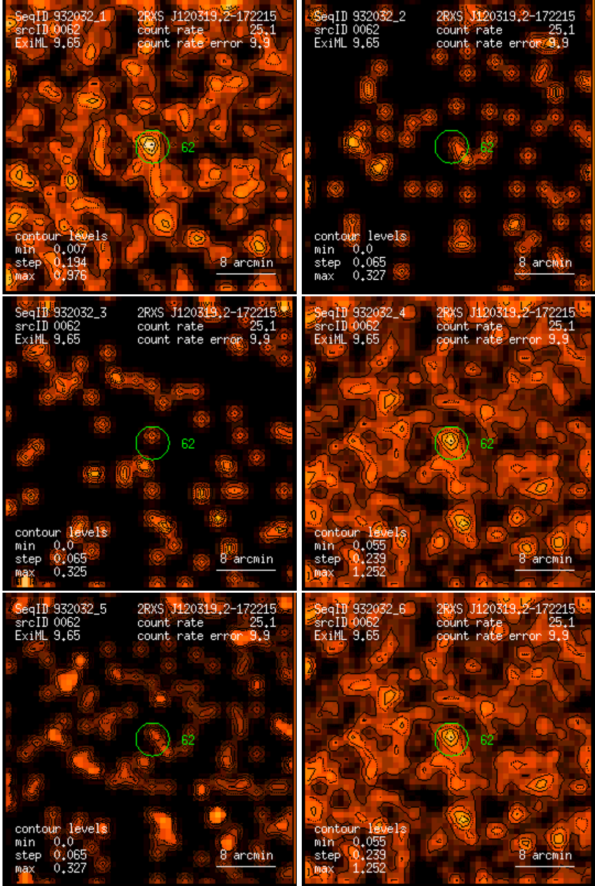
Figure 62: RASS 932032: detection 0062: band rate images, Gaussian filter: (1) PSPC channels 11 – 41, (2) 52 – 90, (3) 91 – 201, (4) 11 – 235, (5) 52 – 201, (6) 11 – 201. Broad band rates in counts/ks. Band rate contour levels in counts/ks/arcmin 2 .
