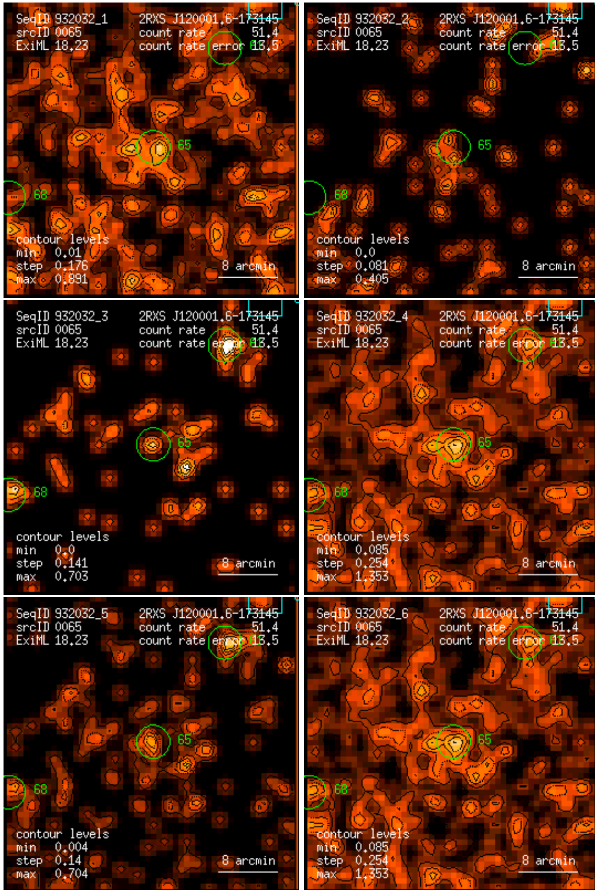
Figure 65: RASS 932032: detection 0065: band rate images, Gaussian filter: (1) PSPC channels 11 – 41, (2) 52 – 90, (3) 91 – 201, (4) 11 – 235, (5) 52 – 201, (6) 11 – 201. Broad band rates in counts/ks. Band rate contour levels in counts/ks/arcmin 2 .
