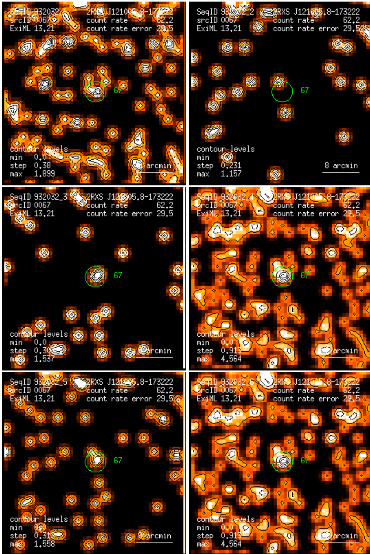
Figure 67: RASS 932032: detection 0067: band rate images, Gaussian filter: (1) PSPC channels 11 – 41, (2) 52 – 90, (3) 91 – 201, (4) 11 – 235, (5) 52 – 201, (6) 11 – 201. Broad band rates in counts/ks. Band rate contour levels in counts/ks/arcmin 2 .
