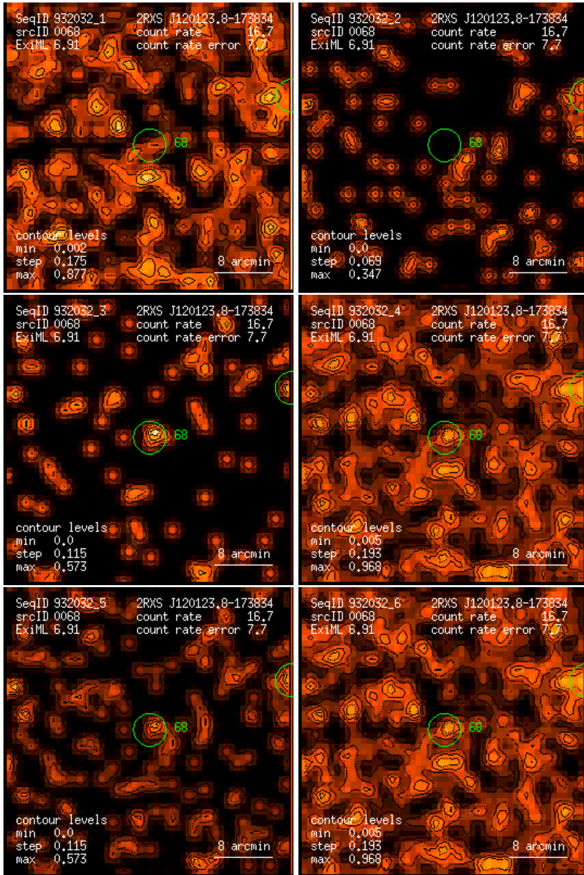
Figure 68: RASS 932032: detection 0068: band rate images, Gaussian filter: (1) PSPC channels 11 – 41, (2) 52 – 90, (3) 91 – 201, (4) 11 – 235, (5) 52 – 201, (6) 11 – 201. Broad band rates in counts/ks. Band rate contour levels in counts/ks/arcmin 2 .
