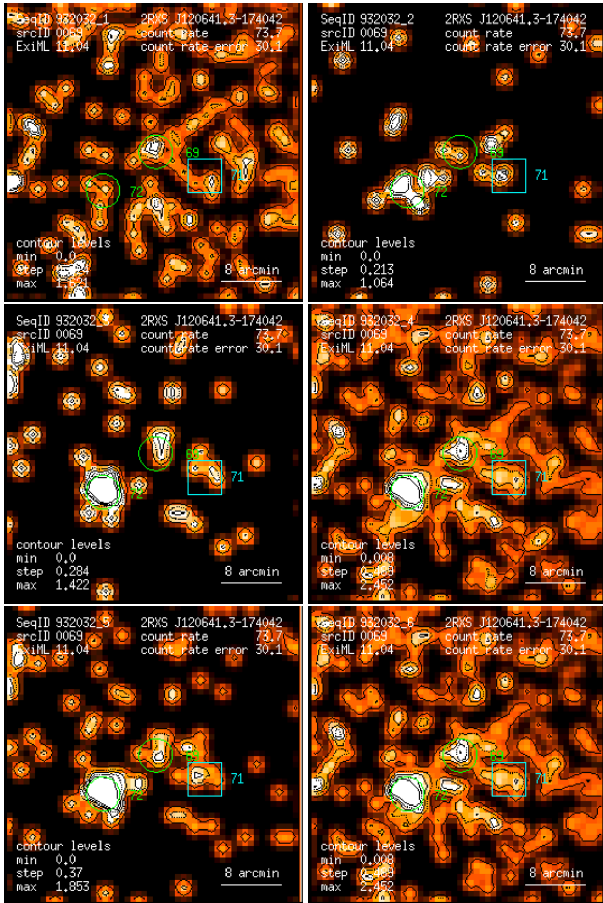
Figure 69: RASS 932032: detection 0069: band rate images, Gaussian filter: (1) PSPC channels 11 – 41, (2) 52 – 90, (3) 91 – 201, (4) 11 – 235, (5) 52 – 201, (6) 11 – 201. Broad band rates in counts/ks. Band rate contour levels in counts/ks/arcmin 2 .
