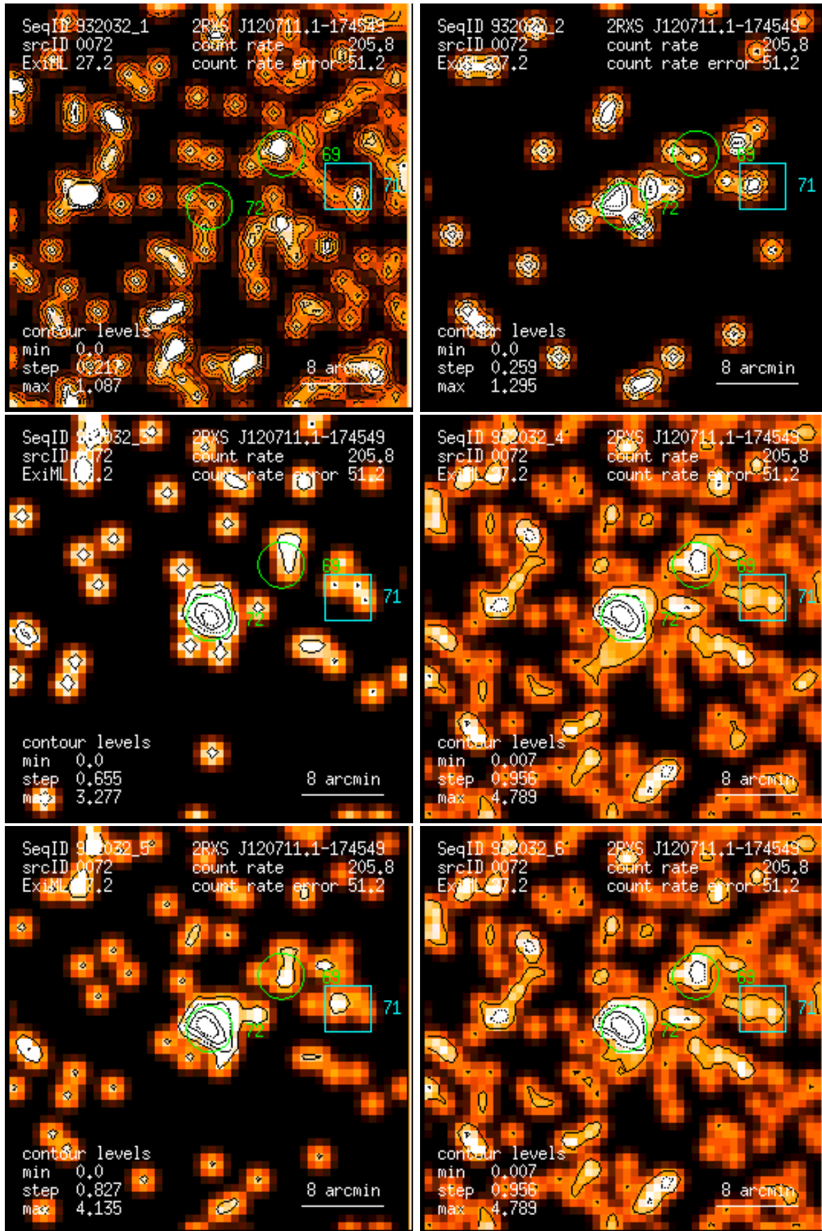
Figure 72: RASS 932032: detection 0072: band rate images, Gaussian filter: (1) PSPC channels 11 – 41, (2) 52 – 90, (3) 91 – 201, (4) 11 – 235, (5) 52 – 201, (6) 11 – 201. Broad band rates in counts/ks. Band rate contour levels in counts/ks/arcmin 2 .
