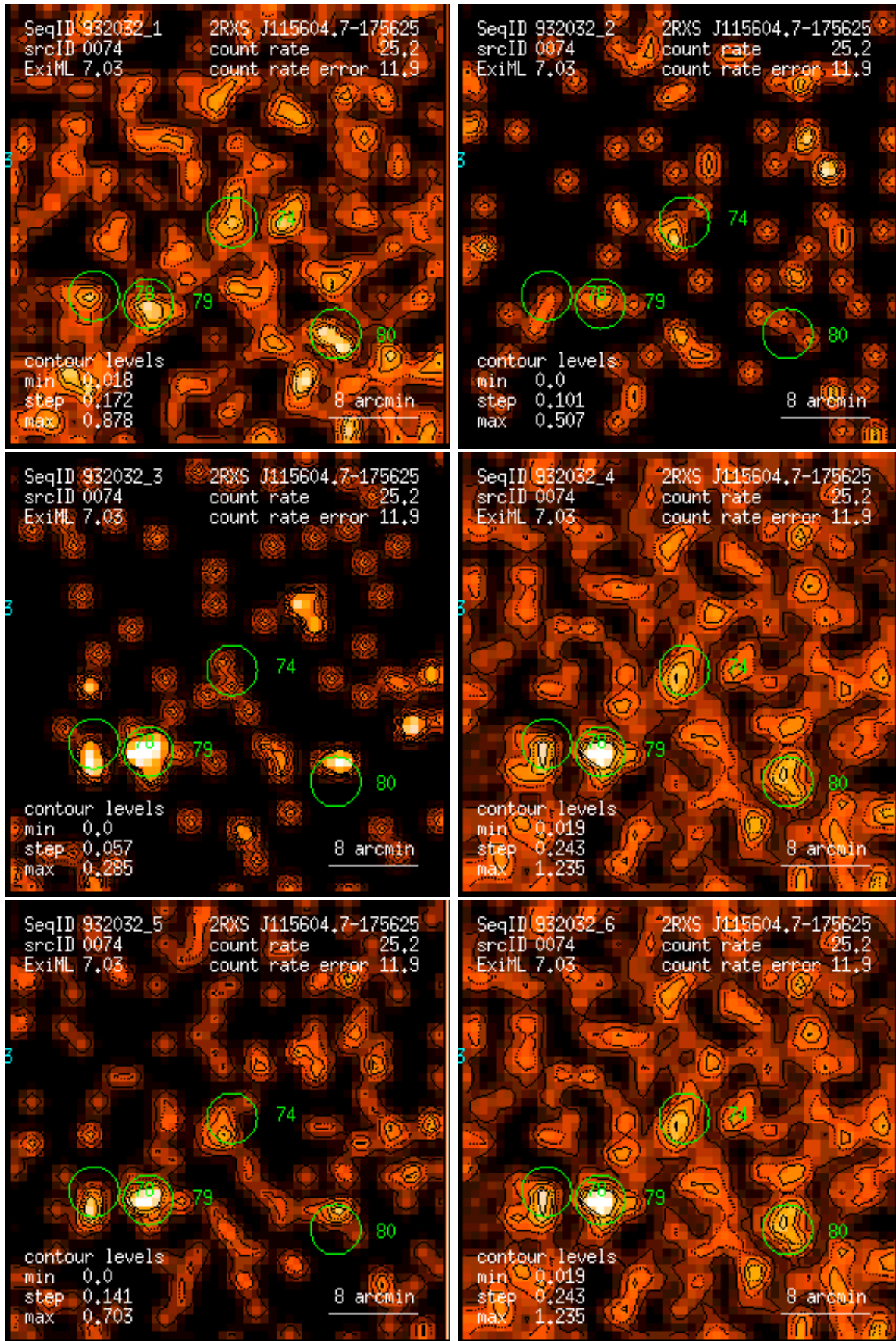
Figure 74: RASS 932032: detection 0074: band rate images, Gaussian filter: (1) PSPC channels 11 – 41, (2) 52 – 90, (3) 91 – 201, (4) 11 – 235, (5) 52 – 201, (6) 11 – 201. Broad band rates in counts/ks. Band rate contour levels in counts/ks/arcmin 2 .
