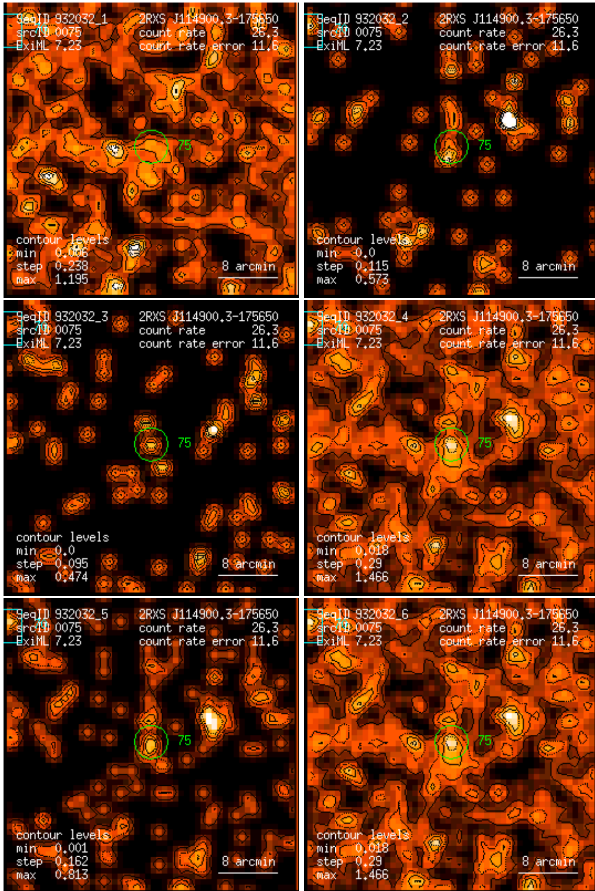
Figure 75: RASS 932032: detection 0075: band rate images, Gaussian filter: (1) PSPC channels 11 – 41, (2) 52 – 90, (3) 91 – 201, (4) 11 – 235, (5) 52 – 201, (6) 11 – 201. Broad band rates in counts/ks. Band rate contour levels in counts/ks/arcmin 2 .
