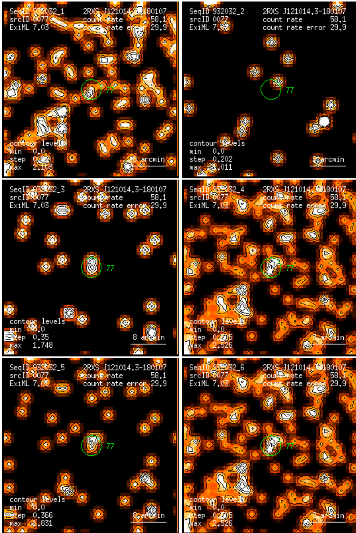
Figure 77: RASS 932032: detection 0077: band rate images, Gaussian filter: (1) PSPC channels 11 – 41, (2) 52 – 90, (3) 91 – 201, (4) 11 – 235, (5) 52 – 201, (6) 11 – 201. Broad band rates in counts/ks. Band rate contour levels in counts/ks/arcmin 2 .
