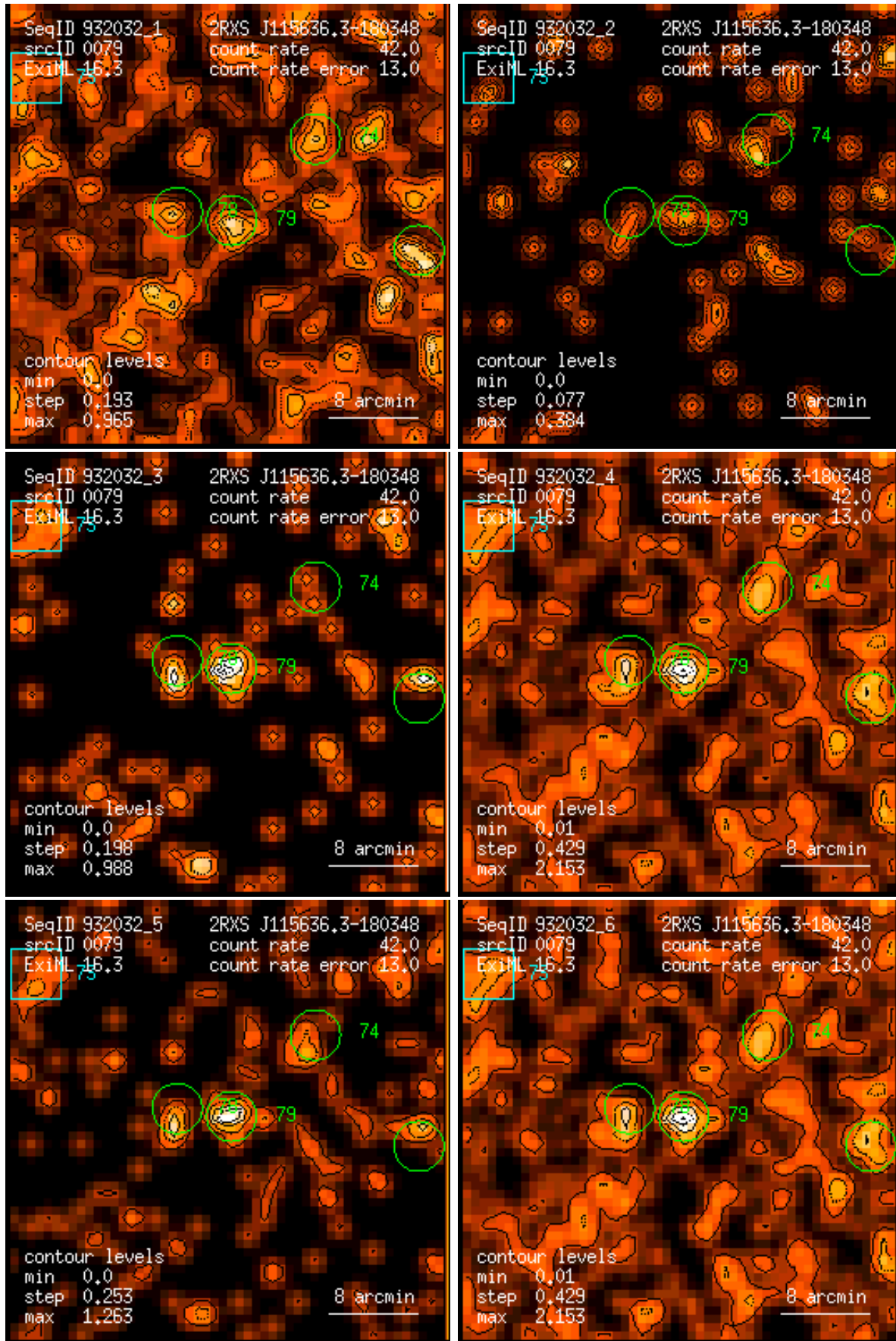
Figure 79: RASS 932032: detection 0079: band rate images, Gaussian filter: (1) PSPC channels 11 – 41, (2) 52 – 90, (3) 91 – 201, (4) 11 – 235, (5) 52 – 201, (6) 11 – 201. Broad band rates in counts/ks. Band rate contour levels in counts/ks/arcmin 2 .
