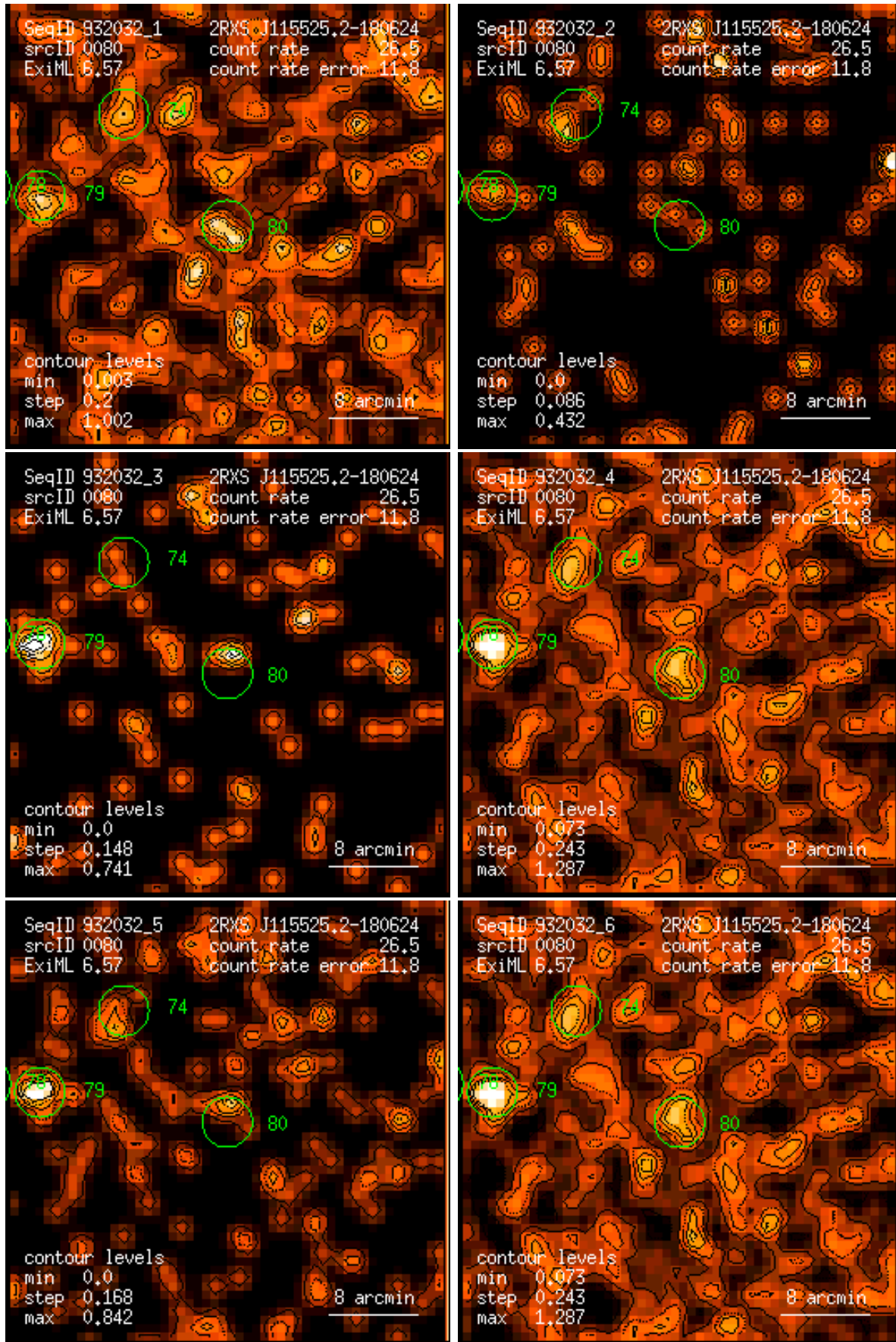
Figure 80: RASS 932032: detection 0080: band rate images, Gaussian filter: (1) PSPC channels 11 – 41, (2) 52 – 90, (3) 91 – 201, (4) 11 – 235, (5) 52 – 201, (6) 11 – 201. Broad band rates in counts/ks. Band rate contour levels in counts/ks/arcmin 2 .
