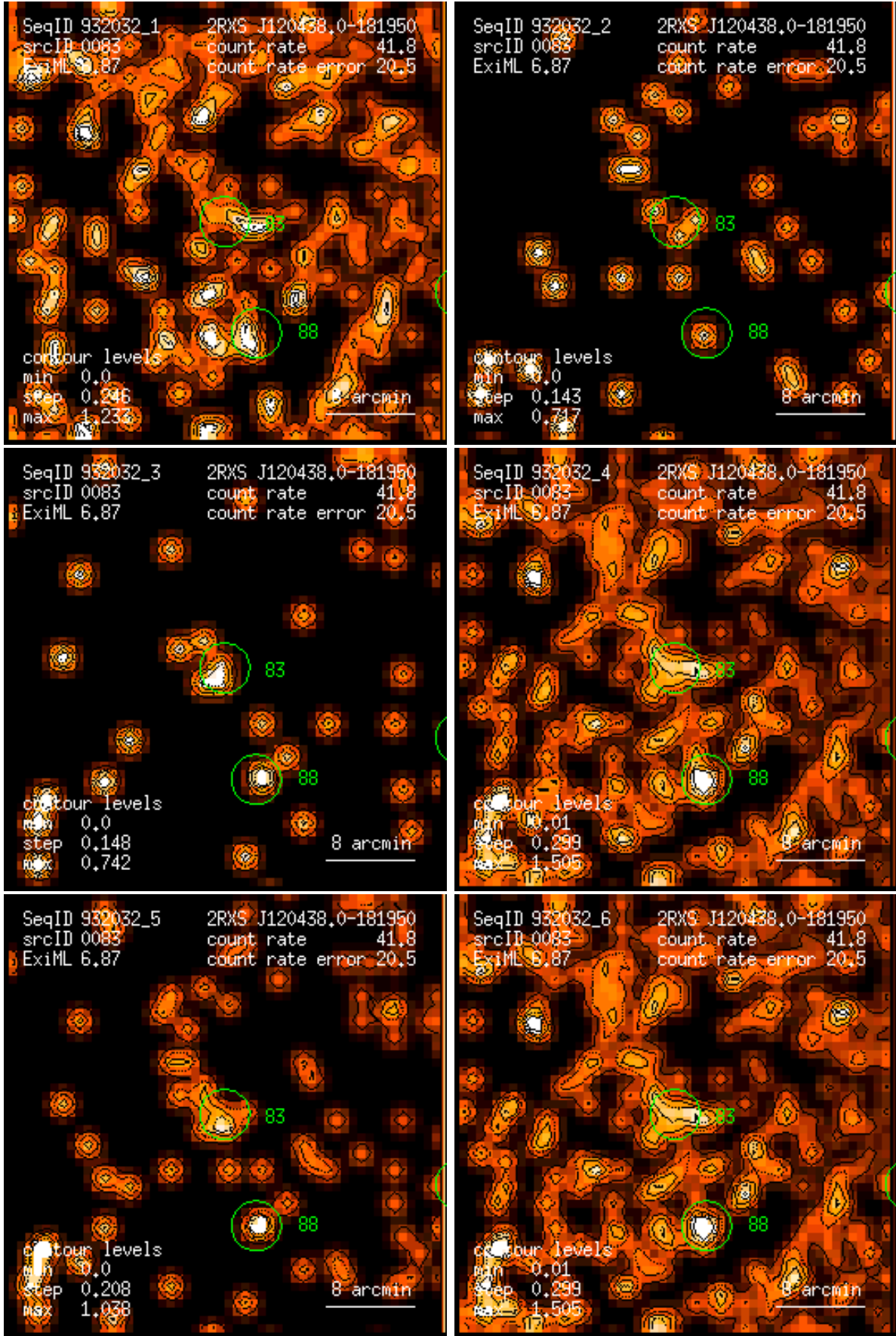
Figure 83: RASS 932032: detection 0083: band rate images, Gaussian filter: (1) PSPC channels 11 – 41, (2) 52 – 90, (3) 91 – 201, (4) 11 – 235, (5) 52 – 201, (6) 11 – 201. Broad band rates in counts/ks. Band rate contour levels in counts/ks/arcmin 2 .
