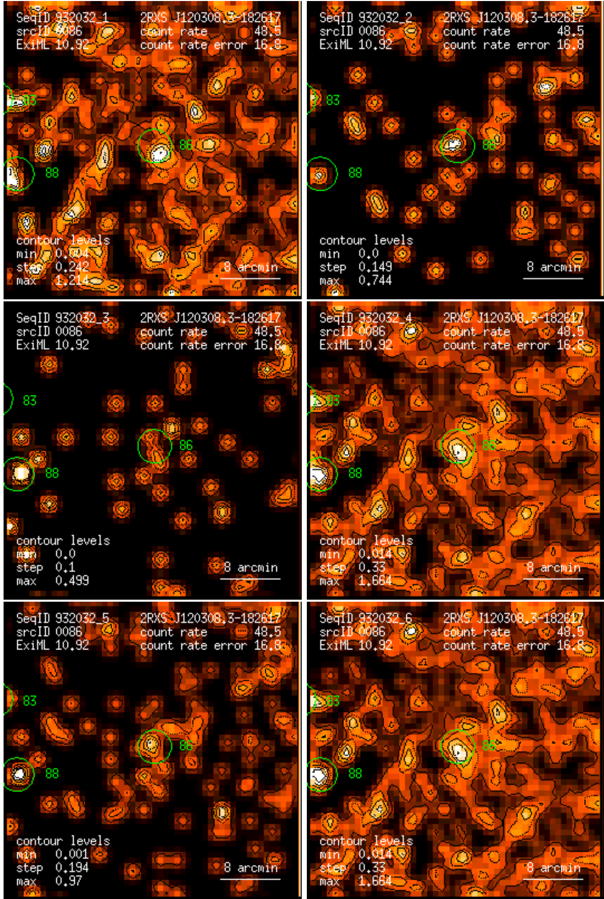
Figure 86: RASS 932032: detection 0086: band rate images, Gaussian filter: (1) PSPC channels 11 – 41, (2) 52 – 90, (3) 91 – 201, (4) 11 – 235, (5) 52 – 201, (6) 11 – 201. Broad band rates in counts/ks. Band rate contour levels in counts/ks/arcmin 2 .
