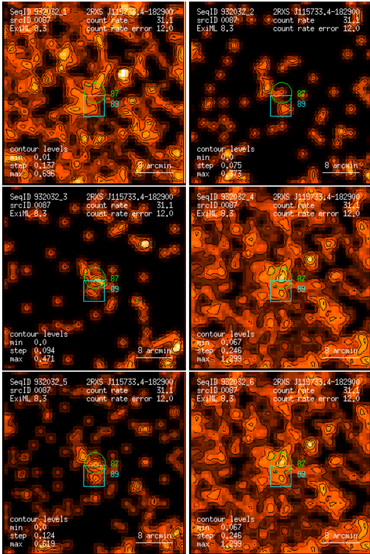
Figure 87: RASS 932032: detection 0087: band rate images, Gaussian filter: (1) PSPC channels 11 – 41, (2) 52 – 90, (3) 91 – 201, (4) 11 – 235, (5) 52 – 201, (6) 11 – 201. Broad band rates in counts/ks. Band rate contour levels in counts/ks/arcmin 2 .
