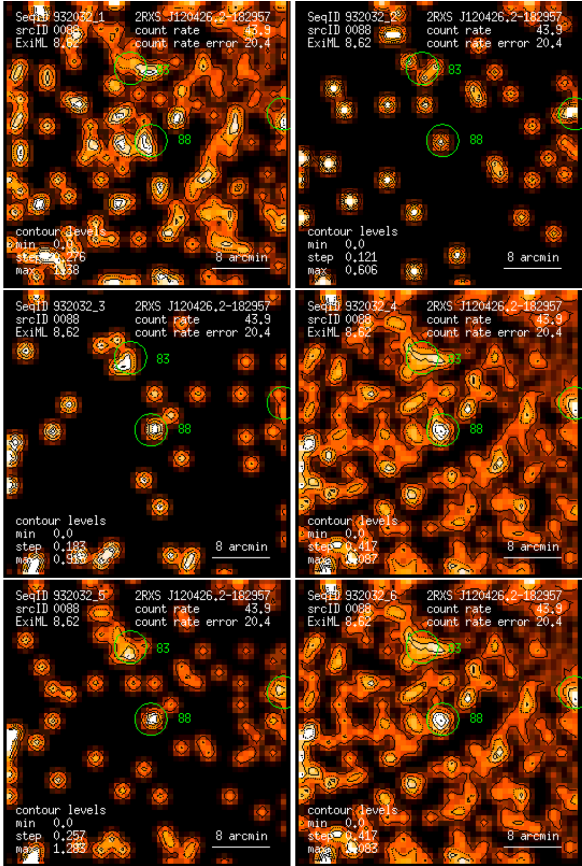
Figure 88: RASS 932032: detection 0088: band rate images, Gaussian filter: (1) PSPC channels 11 – 41, (2) 52 – 90, (3) 91 – 201, (4) 11 – 235, (5) 52 – 201, (6) 11 – 201. Broad band rates in counts/ks. Band rate contour levels in counts/ks/arcmin 2 .
