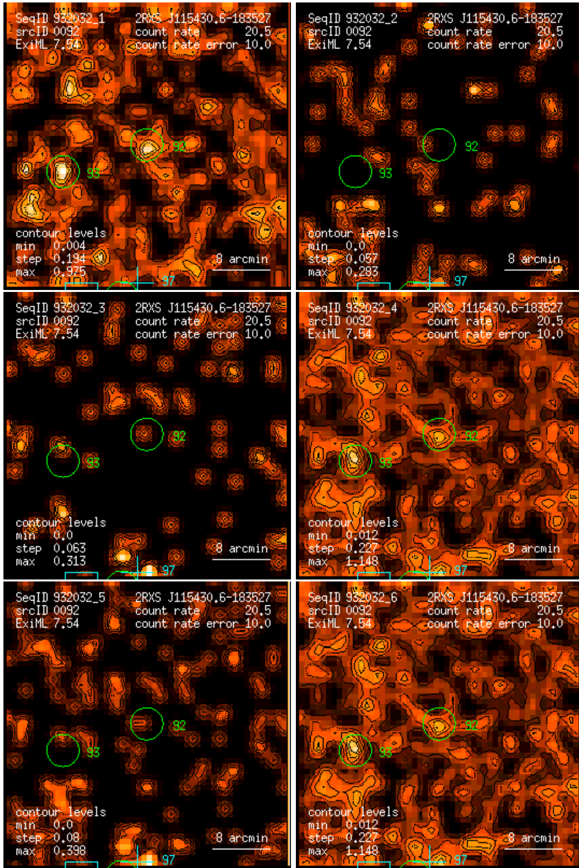
Figure 92: RASS 932032: detection 0092: band rate images, Gaussian filter: (1) PSPC channels 11 – 41, (2) 52 – 90, (3) 91 – 201, (4) 11 – 235, (5) 52 – 201, (6) 11 – 201. Broad band rates in counts/ks. Band rate contour levels in counts/ks/arcmin 2 .
