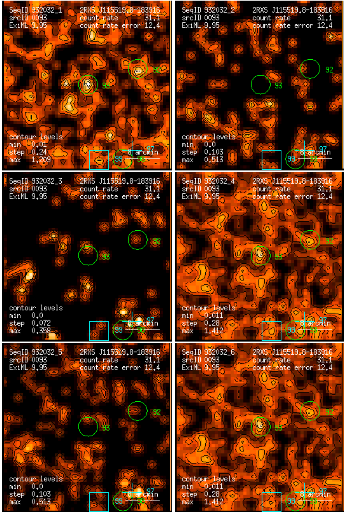
Figure 93: RASS 932032: detection 0093: band rate images, Gaussian filter: (1) PSPC channels 11 – 41, (2) 52 – 90, (3) 91 – 201, (4) 11 – 235, (5) 52 – 201, (6) 11 – 201. Broad band rates in counts/ks. Band rate contour levels in counts/ks/arcmin 2 .
