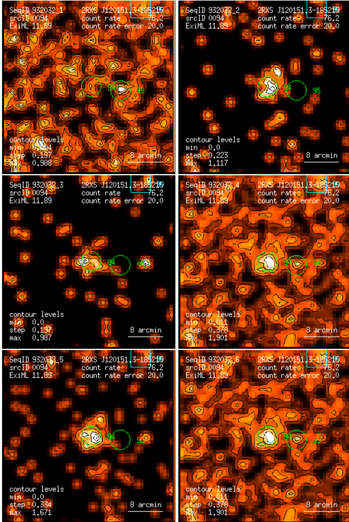
Figure 94: RASS 932032: detection 0094: band rate images, Gaussian filter: (1) PSPC channels 11 – 41, (2) 52 – 90, (3) 91 – 201, (4) 11 – 235, (5) 52 – 201, (6) 11 – 201. Broad band rates in counts/ks. Band rate contour levels in counts/ks/arcmin 2 .
