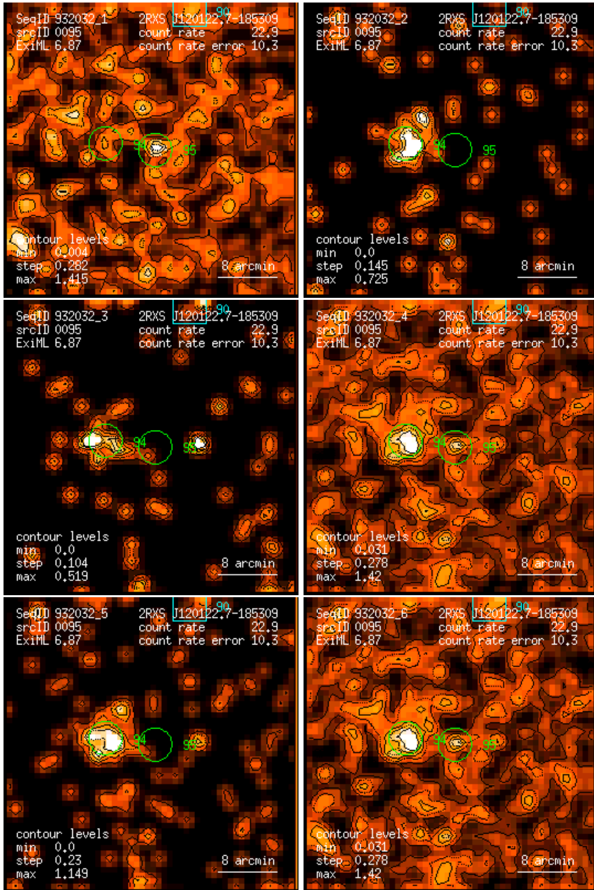
Figure 95: RASS 932032: detection 0095: band rate images, Gaussian filter: (1) PSPC channels 11 – 41, (2) 52 – 90, (3) 91 – 201, (4) 11 – 235, (5) 52 – 201, (6) 11 – 201. Broad band rates in counts/ks. Band rate contour levels in counts/ks/arcmin 2 .
