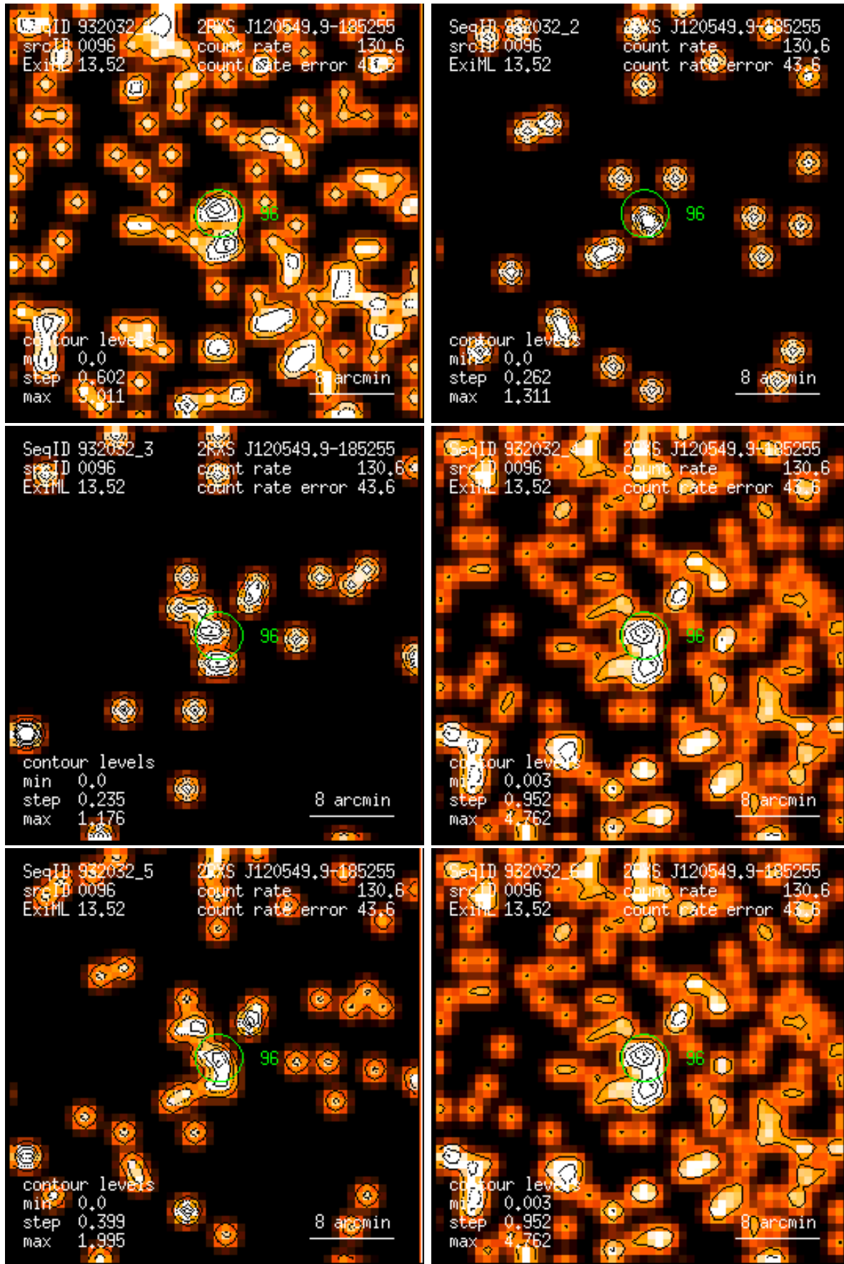
Figure 96: RASS 932032: detection 0096: band rate images, Gaussian filter: (1) PSPC channels 11 – 41, (2) 52 – 90, (3) 91 – 201, (4) 11 – 235, (5) 52 – 201, (6) 11 – 201. Broad band rates in counts/ks. Band rate contour levels in counts/ks/arcmin 2 .
