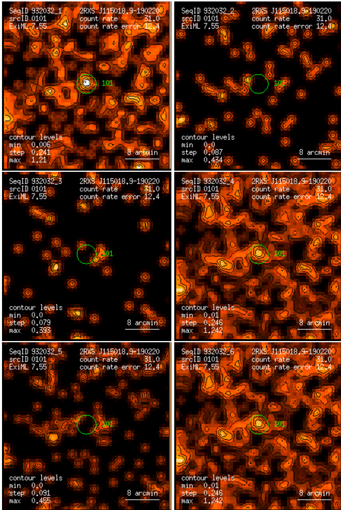
Figure 101: RASS 932032: detection 0101: band rate images, Gaussian filter: (1) PSPC channels 11 – 41, (2) 52 – 90, (3) 91 – 201, (4) 11 – 235, (5) 52 – 201, (6) 11 – 201. Broad band rates in counts/ks. Band rate contour levels in counts/ks/arcmin 2 .
