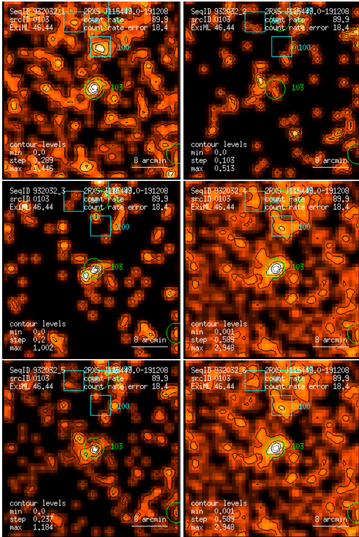
Figure 103: RASS 932032: detection 0103: band rate images, Gaussian filter: (1) PSPC channels 11 – 41, (2) 52 – 90, (3) 91 – 201, (4) 11 – 235, (5) 52 – 201, (6) 11 – 201. Broad band rates in counts/ks. Band rate contour levels in counts/ks/arcmin 2 .
