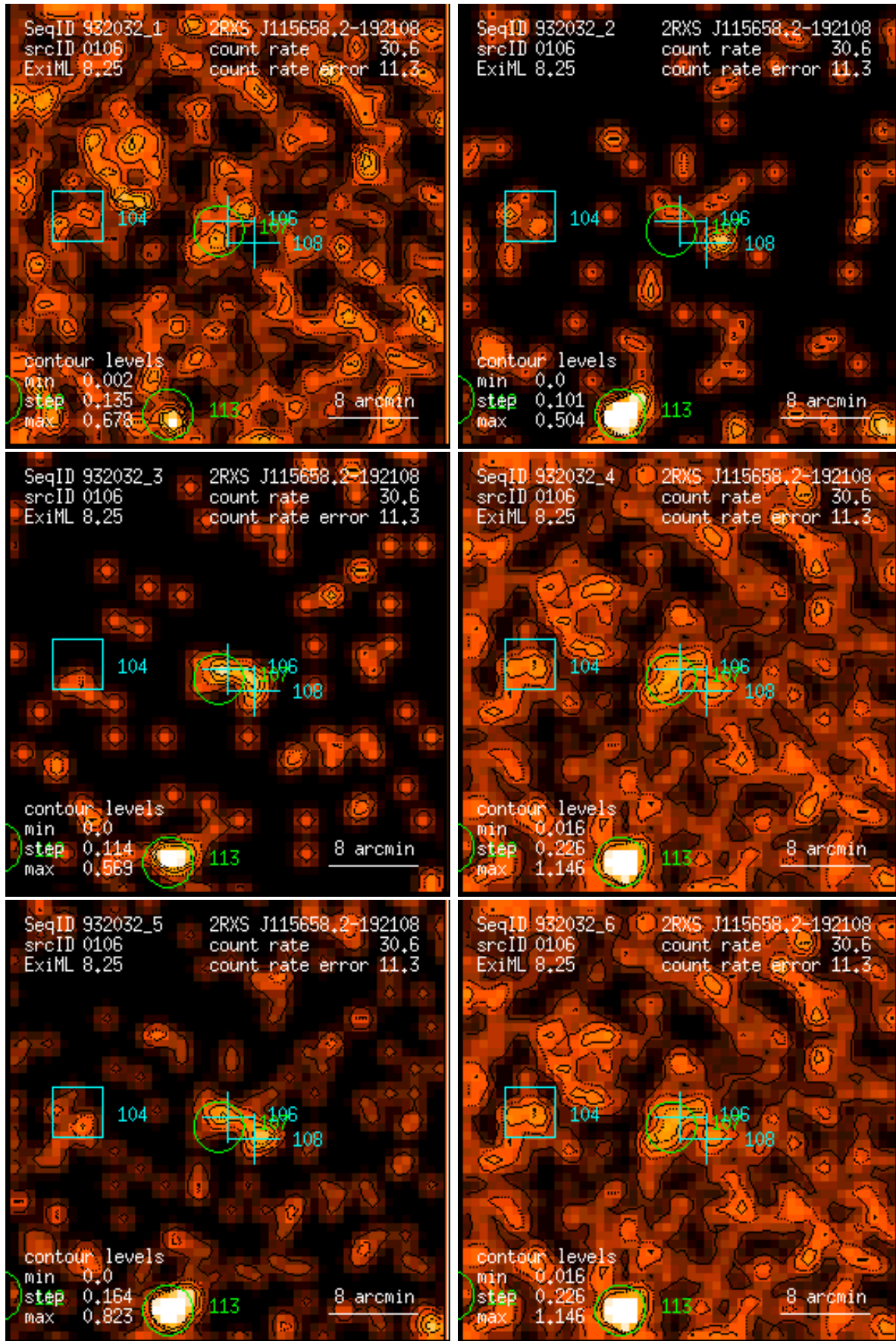
Figure 106: RASS 932032: detection 0106: band rate images, Gaussian filter: (1) PSPC channels 11 – 41, (2) 52 – 90, (3) 91 – 201, (4) 11 – 235, (5) 52 – 201, (6) 11 – 201. Broad band rates in counts/ks. Band rate contour levels in counts/ks/arcmin 2 .
