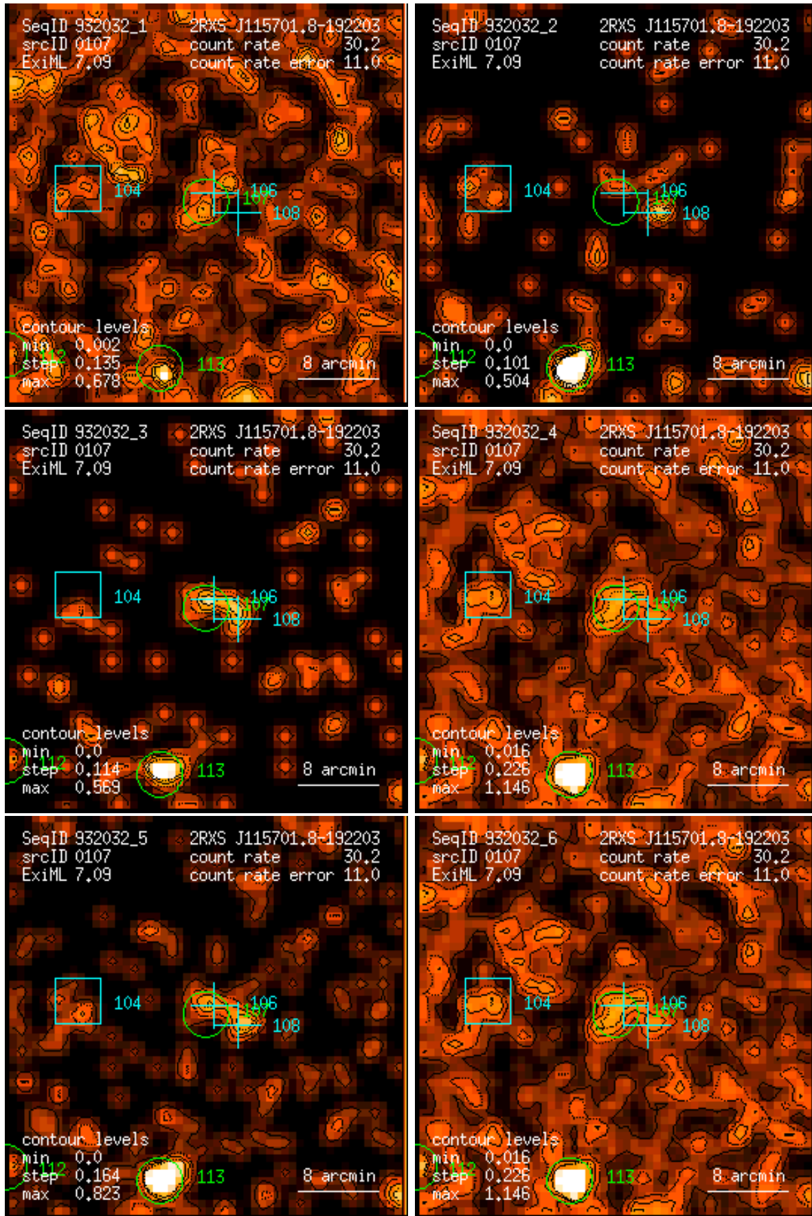
Figure 107: RASS 932032: detection 0107: band rate images, Gaussian filter: (1) PSPC channels 11 – 41, (2) 52 – 90, (3) 91 – 201, (4) 11 – 235, (5) 52 – 201, (6) 11 – 201. Broad band rates in counts/ks. Band rate contour levels in counts/ks/arcmin 2 .
