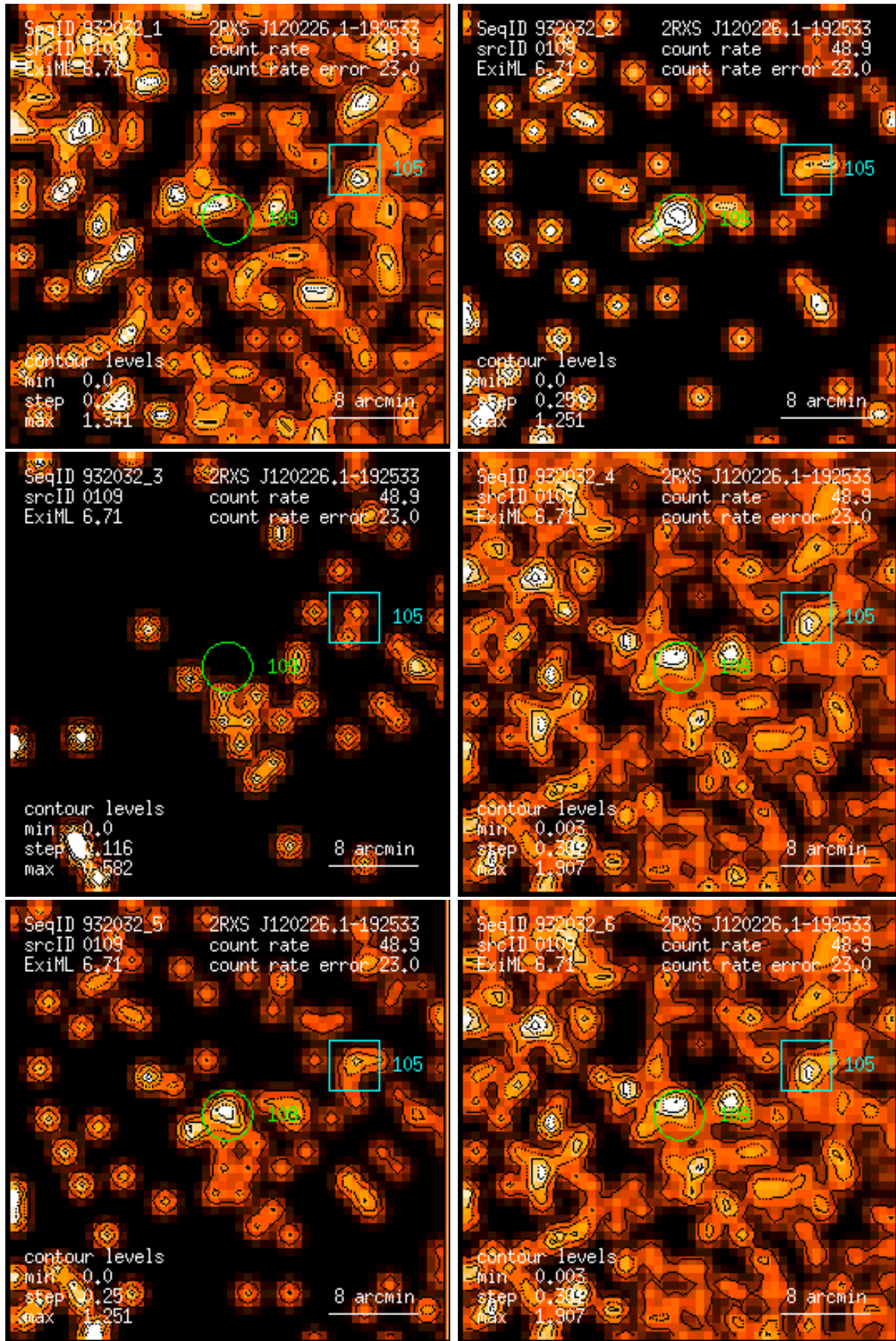
Figure 109: RASS 932032: detection 0109: band rate images, Gaussian filter: (1) PSPC channels 11 – 41, (2) 52 – 90, (3) 91 – 201, (4) 11 – 235, (5) 52 – 201, (6) 11 – 201. Broad band rates in counts/ks. Band rate contour levels in counts/ks/arcmin 2 .
