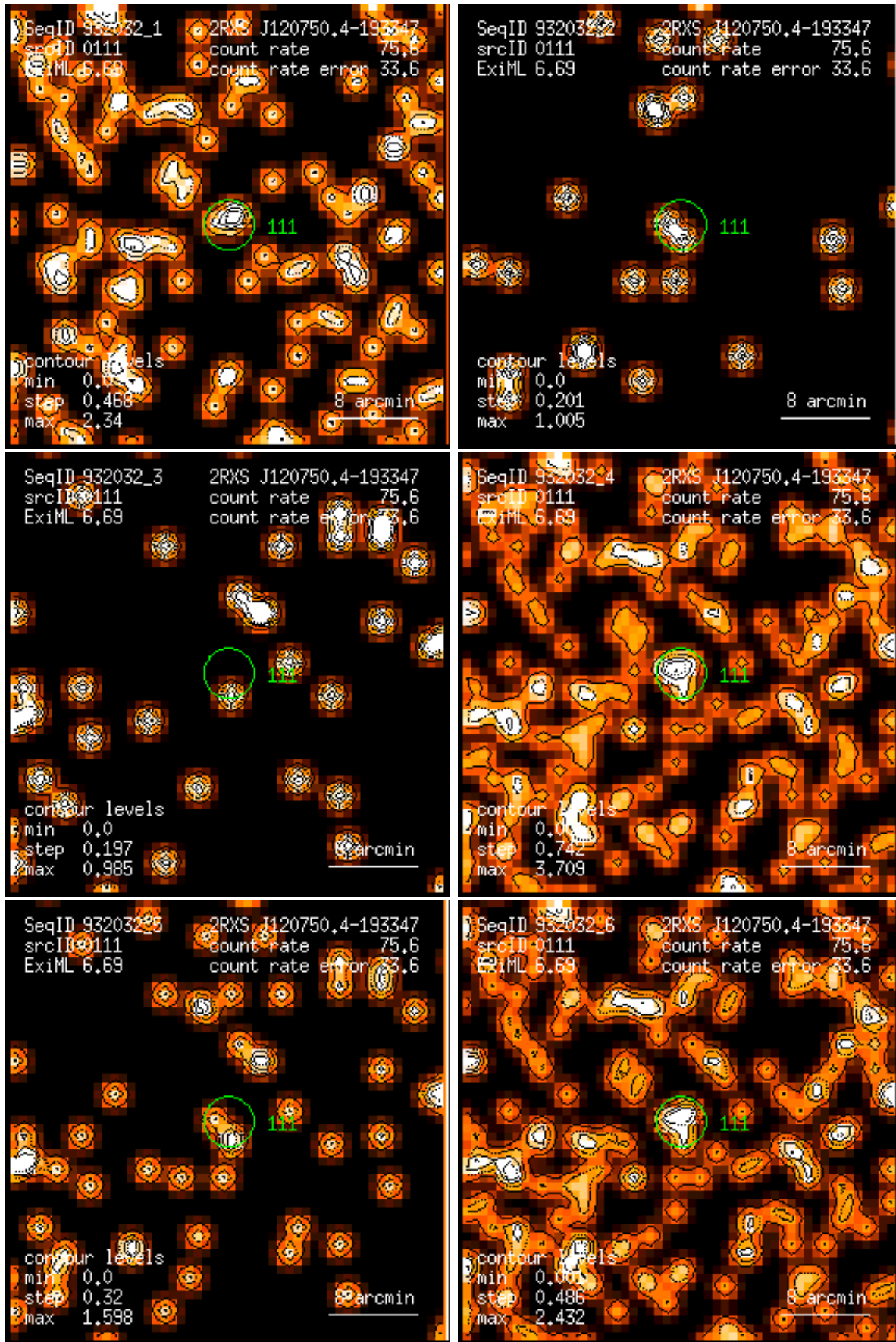
Figure 111: RASS 932032: detection 0111: band rate images, Gaussian filter: (1) PSPC channels 11 – 41, (2) 52 – 90, (3) 91 – 201, (4) 11 – 235, (5) 52 – 201, (6) 11 – 201. Broad band rates in counts/ks. Band rate contour levels in counts/ks/arcmin 2 .
