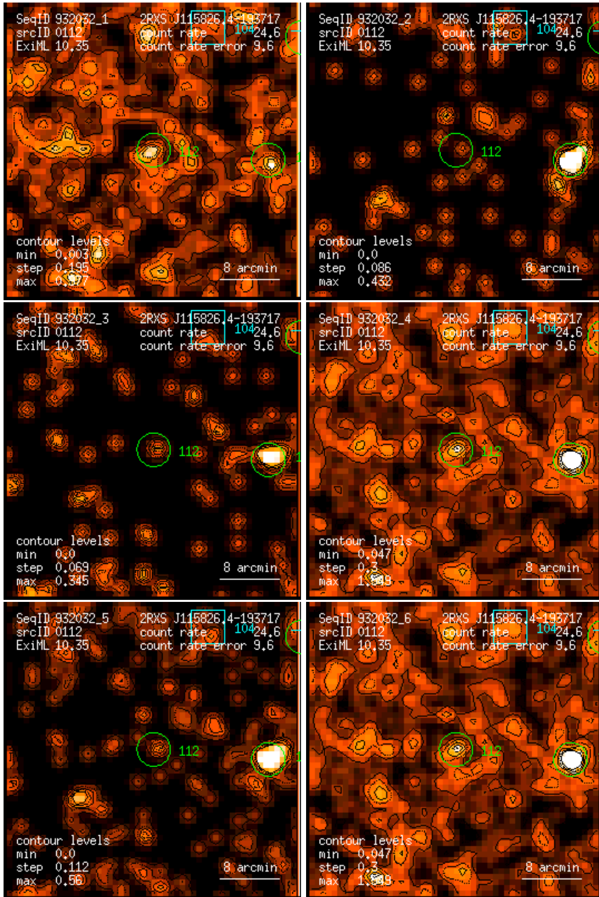
Figure 112: RASS 932032: detection 0112: band rate images, Gaussian filter: (1) PSPC channels 11 – 41, (2) 52 – 90, (3) 91 – 201, (4) 11 – 235, (5) 52 – 201, (6) 11 – 201. Broad band rates in counts/ks. Band rate contour levels in counts/ks/arcmin 2 .
