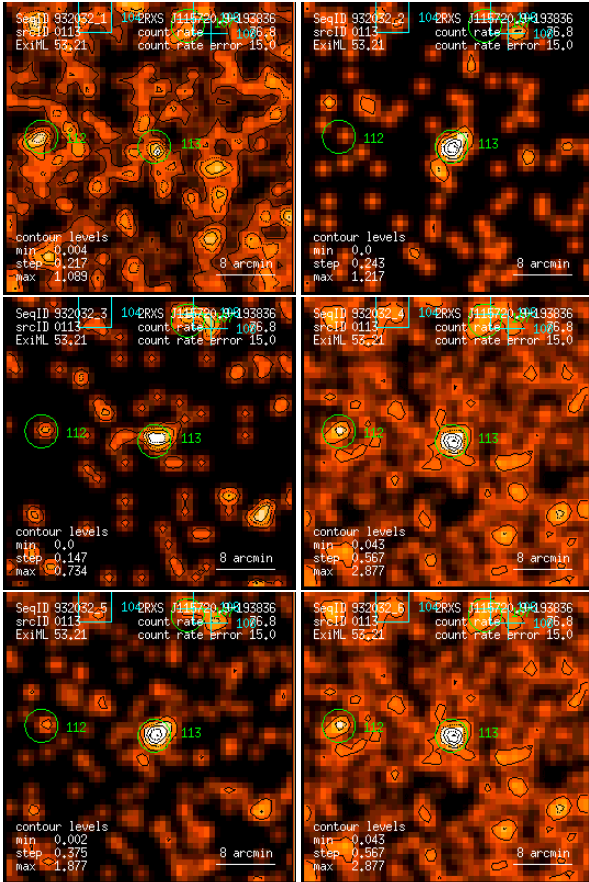
Figure 113: RASS 932032: detection 0113: band rate images, Gaussian filter: (1) PSPC channels 11 – 41, (2) 52 – 90, (3) 91 – 201, (4) 11 – 235, (5) 52 – 201, (6) 11 – 201. Broad band rates in counts/ks. Band rate contour levels in counts/ks/arcmin 2 .
