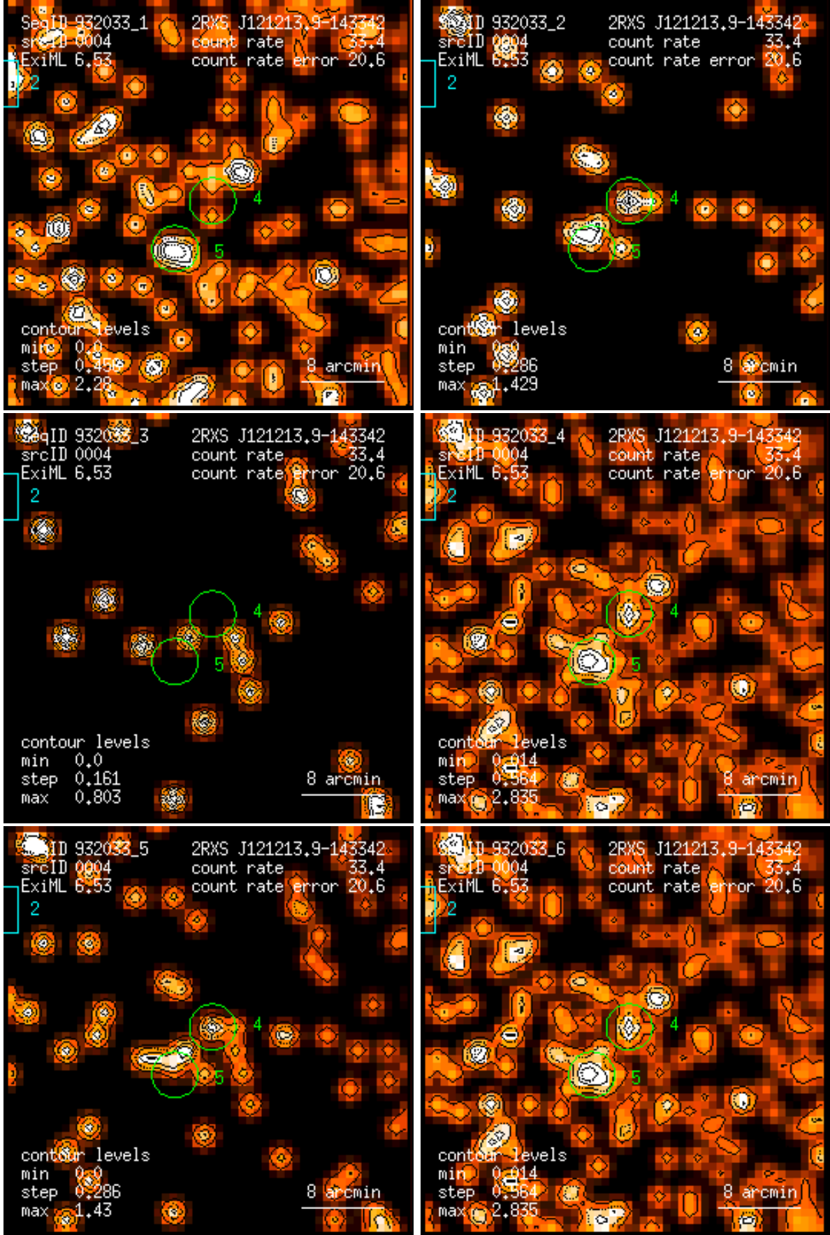
Figure 4: RASS 932033: detection 0004: band rate images, Gaussian filter: (1) PSPC channels 11 – 41, (2) 52 – 90, (3) 91 – 201, (4) 11 – 235, (5) 52 – 201, (6) 11 – 201. Broad band rates in counts/ks. Band rate contour levels in counts/ks/arcmin 2 .
