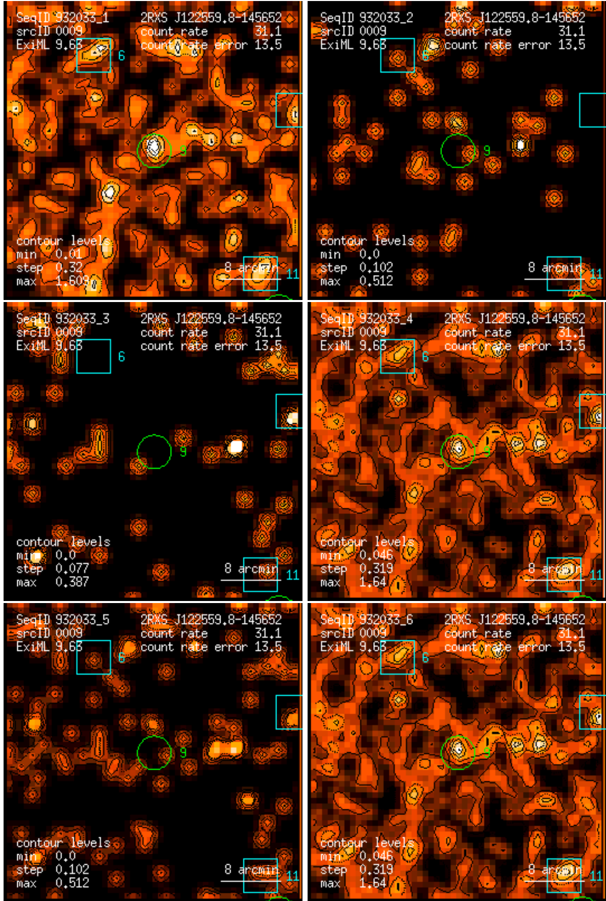
Figure 9: RASS 932033: detection 0009: band rate images, Gaussian filter: (1) PSPC channels 11 – 41, (2) 52 – 90, (3) 91 – 201, (4) 11 – 235, (5) 52 – 201, (6) 11 – 201. Broad band rates in counts/ks. Band rate contour levels in counts/ks/arcmin 2 .
