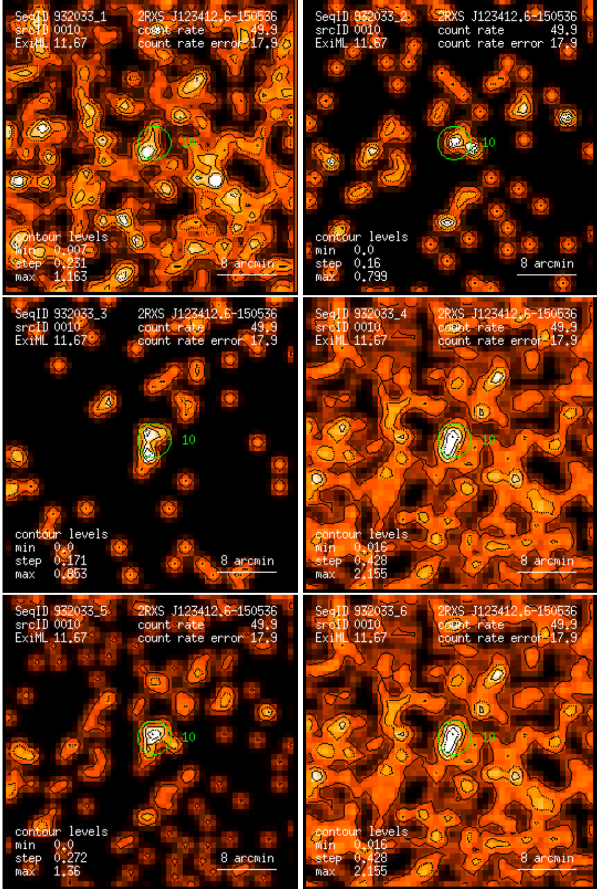
Figure 10: RASS 932033: detection 0010: band rate images, Gaussian filter: (1) PSPC channels 11 – 41, (2) 52 – 90, (3) 91 – 201, (4) 11 – 235, (5) 52 – 201, (6) 11 – 201. Broad band rates in counts/ks. Band rate contour levels in counts/ks/arcmin 2 .
