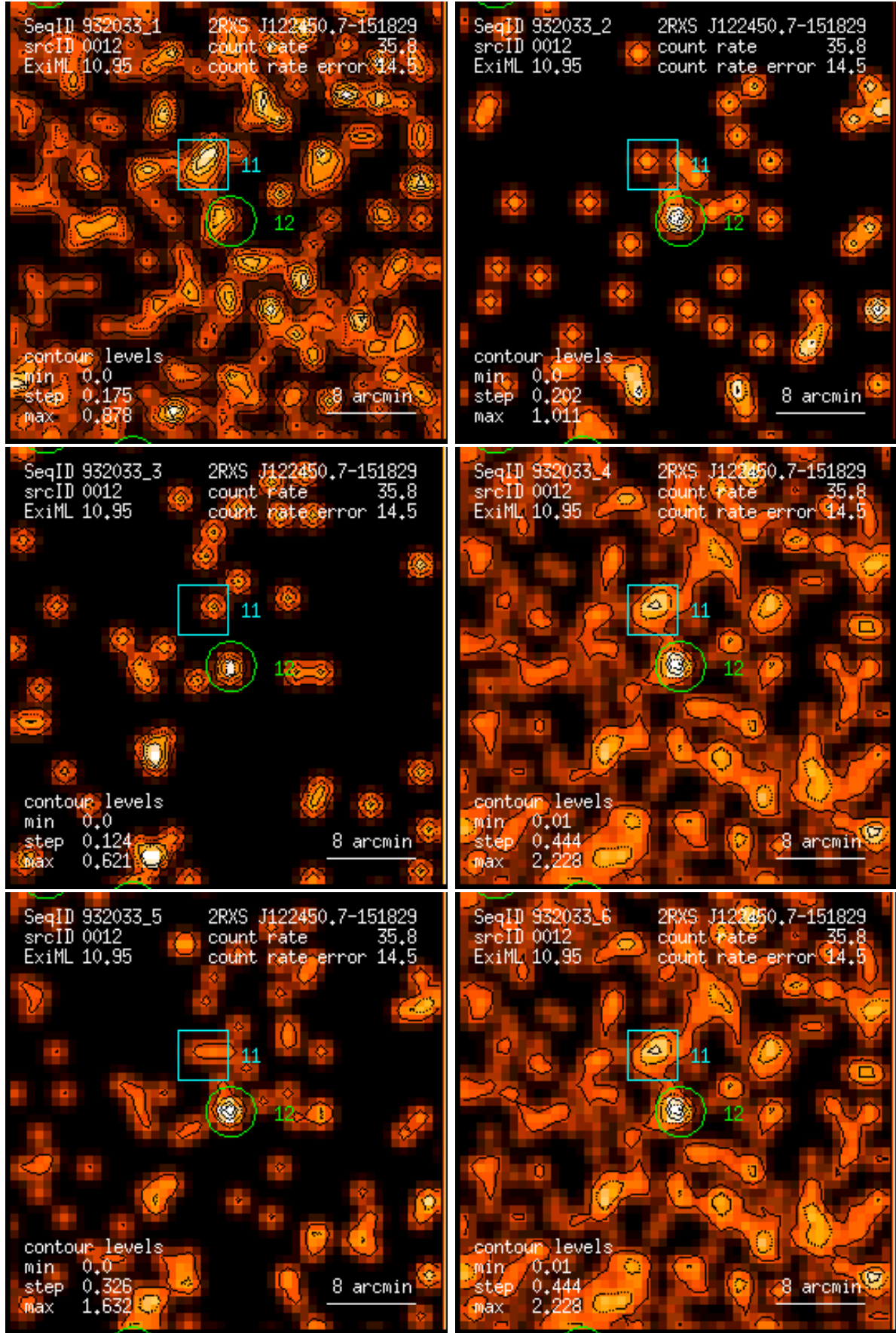
Figure 12: RASS 932033: detection 0012: band rate images, Gaussian filter: (1) PSPC channels 11 – 41, (2) 52 – 90, (3) 91 – 201, (4) 11 – 235, (5) 52 – 201, (6) 11 – 201. Broad band rates in counts/ks. Band rate contour levels in counts/ks/arcmin 2 .
