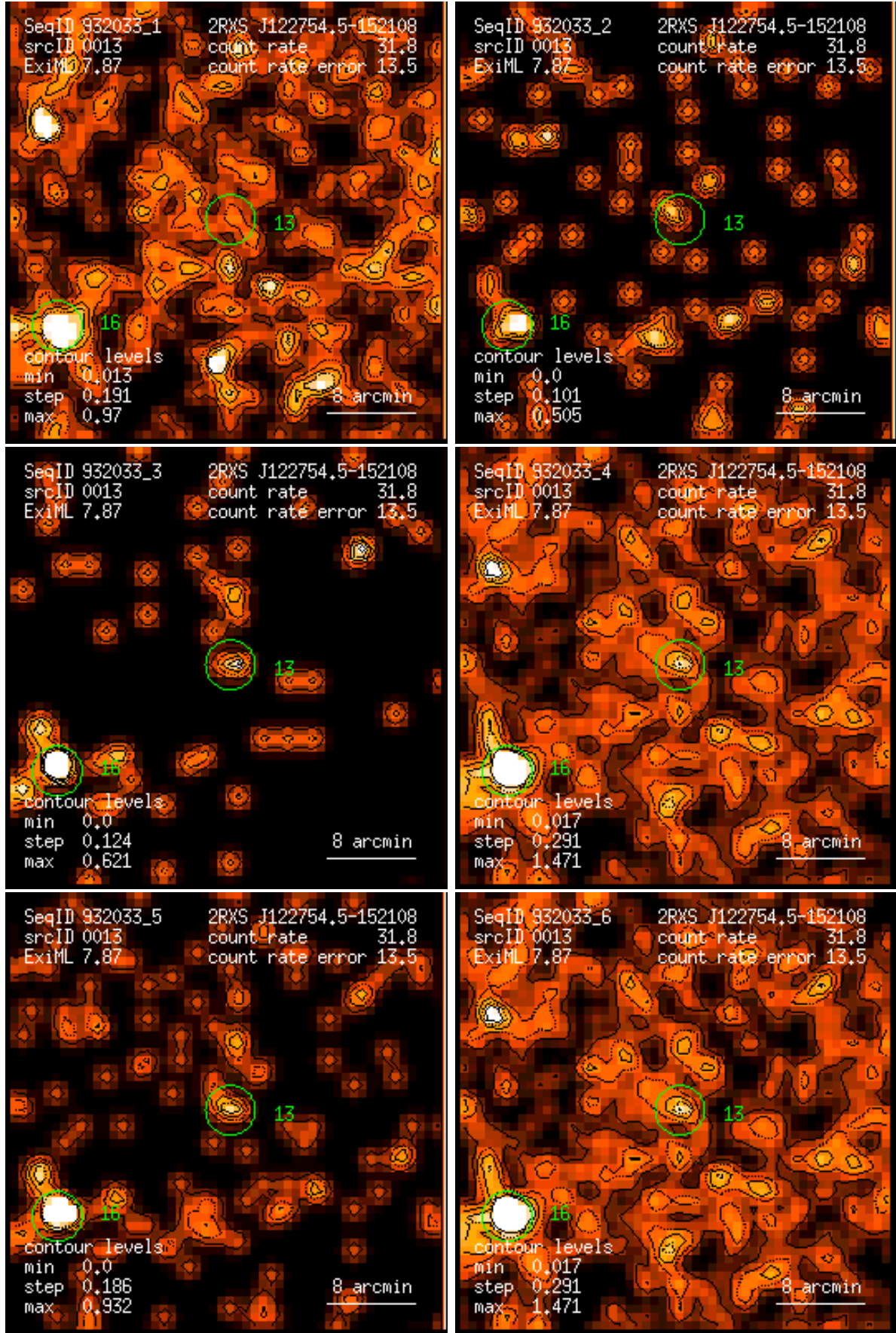
Figure 13: RASS 932033: detection 0013: band rate images, Gaussian filter: (1) PSPC channels 11 – 41, (2) 52 – 90, (3) 91 – 201, (4) 11 – 235, (5) 52 – 201, (6) 11 – 201. Broad band rates in counts/ks. Band rate contour levels in counts/ks/arcmin 2 .
