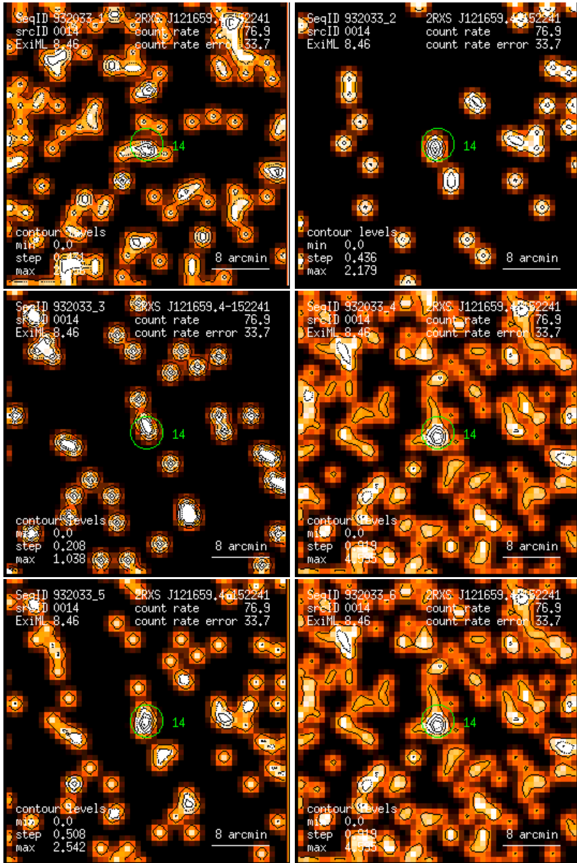
Figure 14: RASS 932033: detection 0014: band rate images, Gaussian filter: (1) PSPC channels 11 – 41, (2) 52 – 90, (3) 91 – 201, (4) 11 – 235, (5) 52 – 201, (6) 11 – 201. Broad band rates in counts/ks. Band rate contour levels in counts/ks/arcmin 2 .
