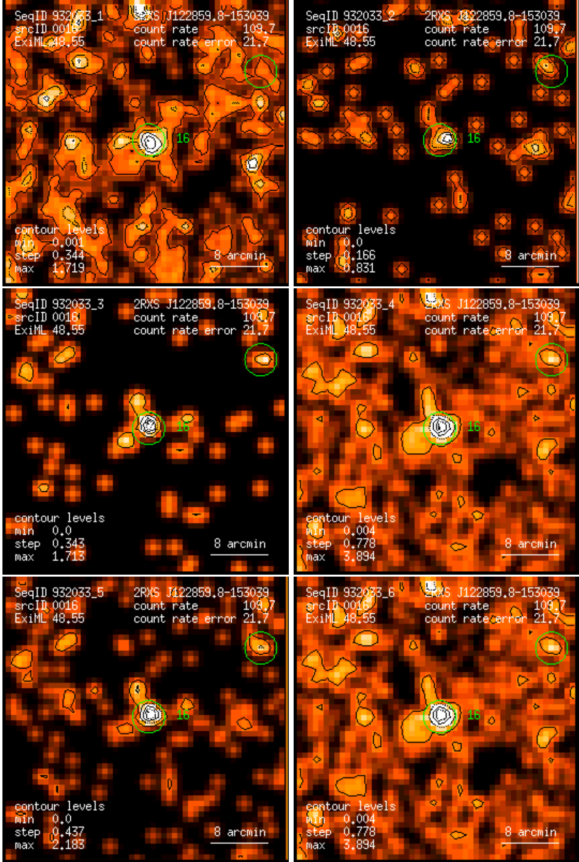
Figure 16: RASS 932033: detection 0016: band rate images, Gaussian filter: (1) PSPC channels 11 – 41, (2) 52 – 90, (3) 91 – 201, (4) 11 – 235, (5) 52 – 201, (6) 11 – 201. Broad band rates in counts/ks. Band rate contour levels in counts/ks/arcmin 2 .
