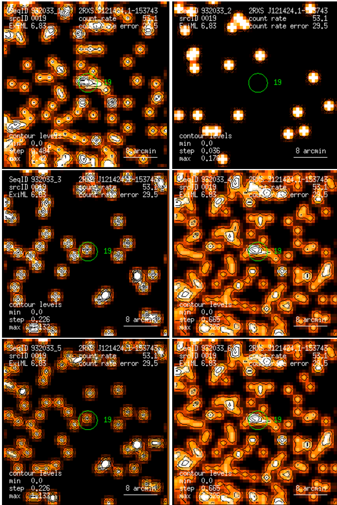
Figure 19: RASS 932033: detection 0019: band rate images, Gaussian filter: (1) PSPC channels 11 – 41, (2) 52 – 90, (3) 91 – 201, (4) 11 – 235, (5) 52 – 201, (6) 11 – 201. Broad band rates in counts/ks. Band rate contour levels in counts/ks/arcmin 2 .
